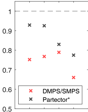
\rho_{\text{eff}} corrected
