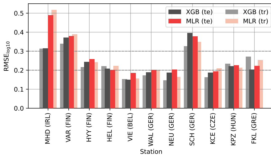
Figure S2. The comparison between MLR and XGB station-excluded model testing and training errors (RMSE calculated for log10-transformed concentrations) for the stations that had data during 2020-2022.
