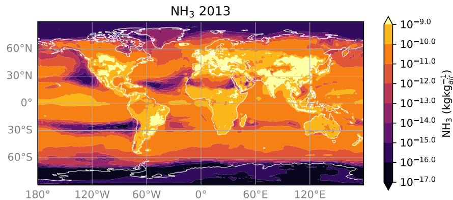
Figure S6. Average ammonia concentration in 2013. The low ammonia concentrations result in low N100 estimate with MLR global model.
