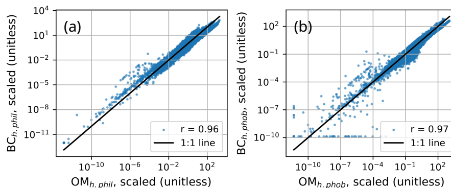
Figure S4. In the training set, the Pearson correlation coefficient ( r ) was very high between BC mixing ratio and OM mixing ratio both for a) hydrophilic mixing ratios and b) hydrophobic mixing ratios. The figure shows the scaled values.
