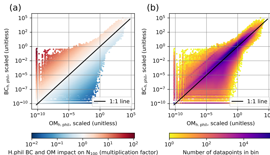
Figure S5. Panel a) shows the combined contribution of BC_{h,phil} and OM_{h,phil} to the total N100. Panel b) shows how the data points are distributed.
