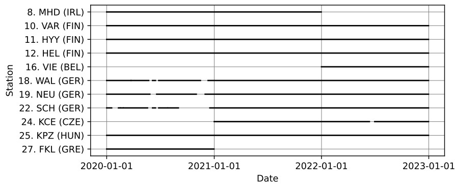
Figure S1. The data-availability of N100 measurements in the holdout set.
