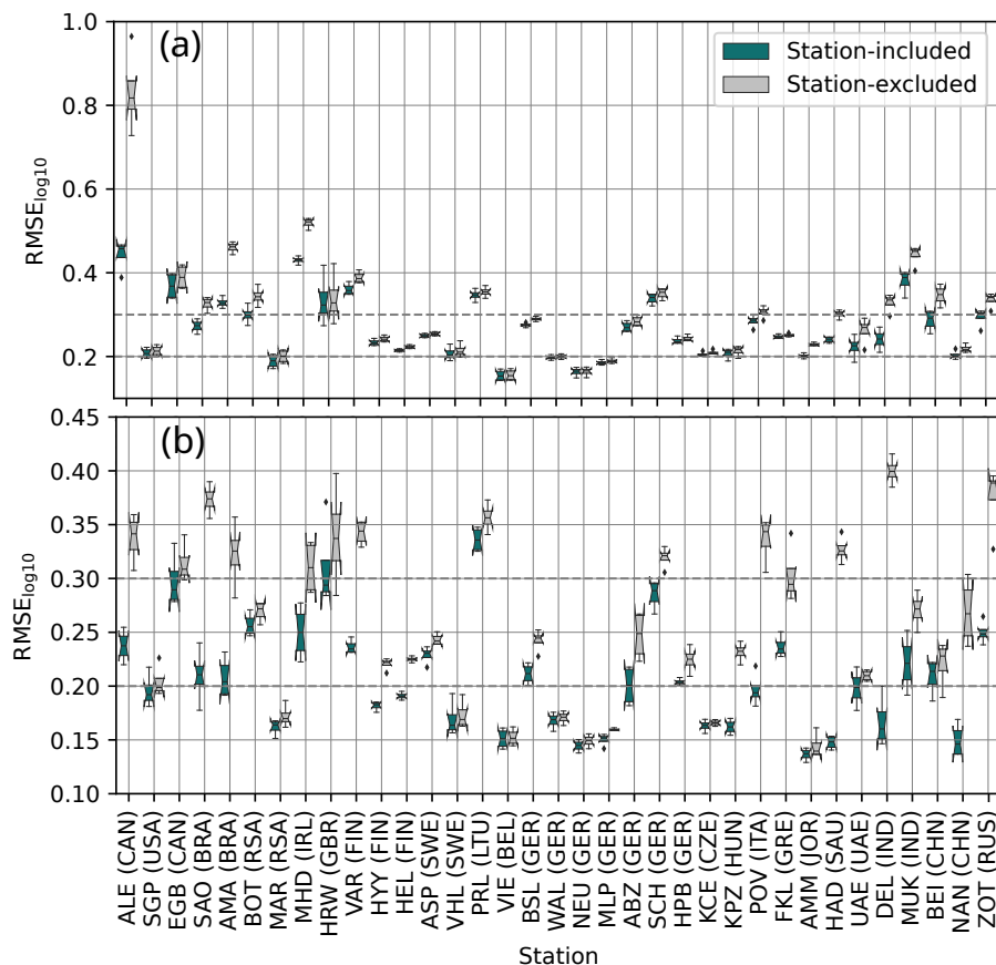
Figure S3. Boxplots comparing the model performance (RMSE calculated for log10-transformed concentrations) of station-included and station-excluded a) MLR models b) XGB models at each station. For this analysis we modified the station-excluded models to have validation sets corresponding to station-included models (Table 3). The boxes indicate the variation caused by different train-validation splits. The boxes show the quartiles and whiskers show the 1.5 interquartile range of the lower and upper quartile. Data points outside these are considered outliers and marked with individual markers. Additionally notches in the boxplots indicate the confidence interval of the median. If the notches of two boxes do not overlap, it indicates that the medians are statistically significantly different at 5 % significance level.
