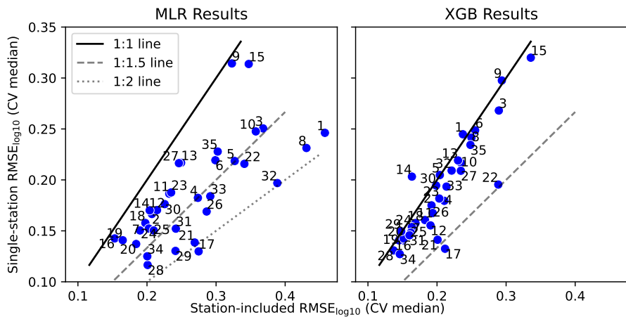
Figure S7. The comparison between the medians of cross-validation (CV) results from single-station and station-included models for a) MLR and b) XGB. The numbers correspond to stations as listed in Table 1.
