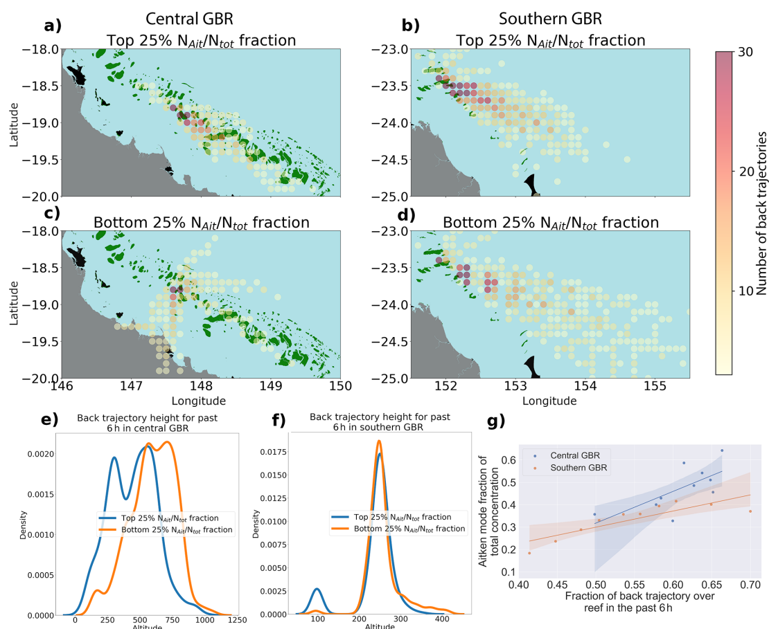
Figure 6. Spatial distribution of 6 h back trajectories for data with top 25 percentile (a, b) and bottom 25 percentile (c, d) of Aitken-mode fraction in proportion to total particle concentration in central GBR (left) and southern GBR (right). The green areas are reefs, black areas are islands, and the grey area is the Australian mainland. Kernel density estimates for the back trajectory altitude for top 25 % (blue) and bottom 25 % (orange) Aitken-mode fraction in central (e) and southern (f) GBR. Fraction of the total aerosol number concentration in the Aitken mode plotted against the proportion of the past 6 h during which the air mass was over the reef at central and southern GBR (g). The lines are linear fits to calculated Aitken-mode fraction quantiles and their respective reef fractions. Shaded areas represent the line fit uncertainty.
