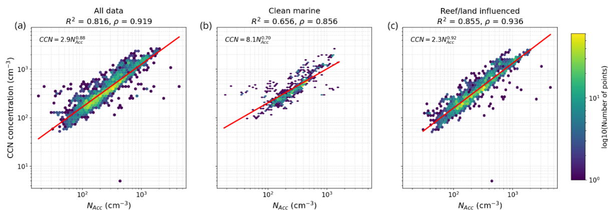
Figure 5. An ordinary least squares regression analysis fitted to log-log accumulation mode ( N_{ACC} ) and CCN concentration data for all the data (a), clean marine data (b), and reef/land-influenced data.
