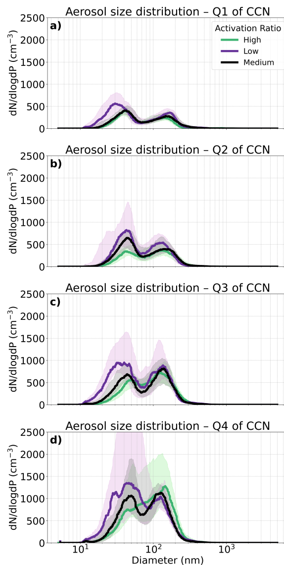
Figure 3. Aerosol size distributions for the four quartiles of CCN concentrations (a, b, c, d). Aerosol size distributions are coloured by the activation ratio low (0.03–0.53; purple), medium (0.53–0.69; black), and high (0.69–0.99; green). Shaded areas present the interquartile ranges. Values of activation ratio ranges for each CCN concentration quartile as well as values of CCN concentration quartile are listed in Table S3.
