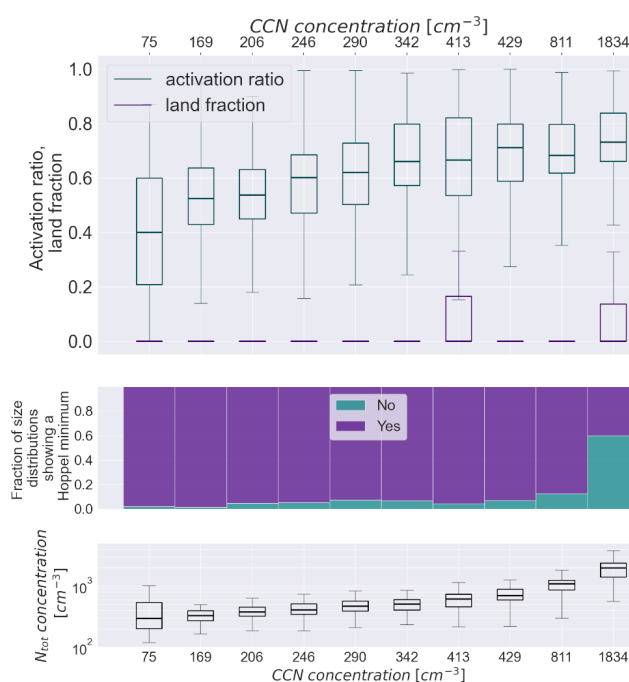
Figure 2. Activation ratio, land fraction, and fraction of data with no Hoppel minimum present as well as total number concentration of particles for different CCN concentration bins. CCN concentration bins were created based on CCN concentration quantiles, ensuring equal distribution of data points between analysed bins. Values of activation ratio, land fraction, and total number concentration of particles are visualized by boxplots. Here, the middle line represents the median value; the upper and lower edges of a box show 75 % and 25 % percentiles, respectively; and the whiskers show the entire range.
