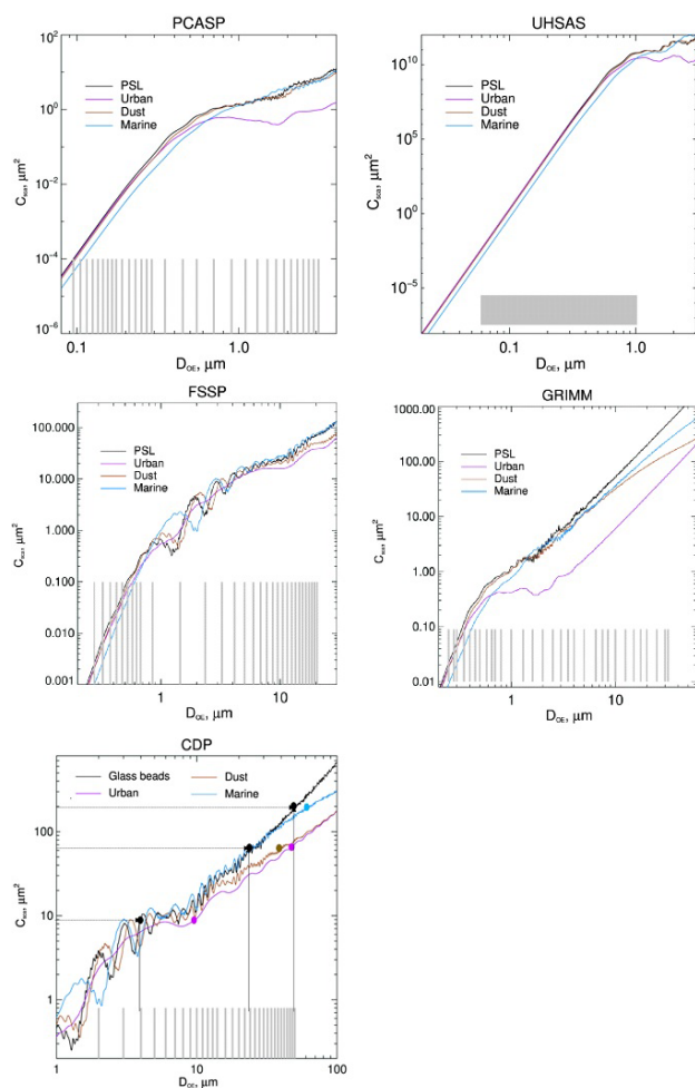
Figure 2. Scattering cross-section C_{\text{sca}} as a function of particle diameter calculated using Mie theory for the OPCs considered in this paper. The black lines represent C_{\text{sca}} for the calibration particles (PSL or glass beads). The purple lines represent the C_{\text{sca}} function for absorbing urban aerosols ( m = 1.56 - 0.087i ), while the brown lines represent C_{\text{sca}} for moderately absorbing mineral dust ( m = 1.53 - 0.003i ), and the light-blue lines represent C_{\text{sca}} for marine aerosols ( m = 1.38 - 0.001i ). The small vertical gray lines represent the bin edges for each OPC.
