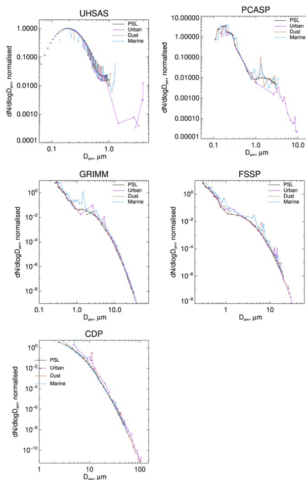
Figure 4. Representation of a bimodal lognormal size distribution by the OPCs considered in this paper, taking into account the corrected bin diameter for the example aerosol types (mineral dust, urban and marine).
