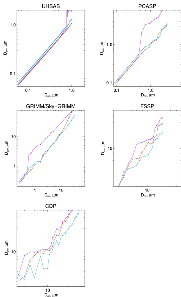
Figure 3. For each OPC: scatterplot of geometric-equivalent bin size boundary ( D_{\text{geo}} ) corresponding to the complex refractive index of the example aerosol types (mineral dust, urban and marine) with respect to the optical-equivalent bin size boundary ( D_{\text{OE}} ) obtained if the calibration m is used. The color code is a light-blue line for marine aerosol, a purple line for urban aerosol, and a brown line for mineral dust aerosol.
