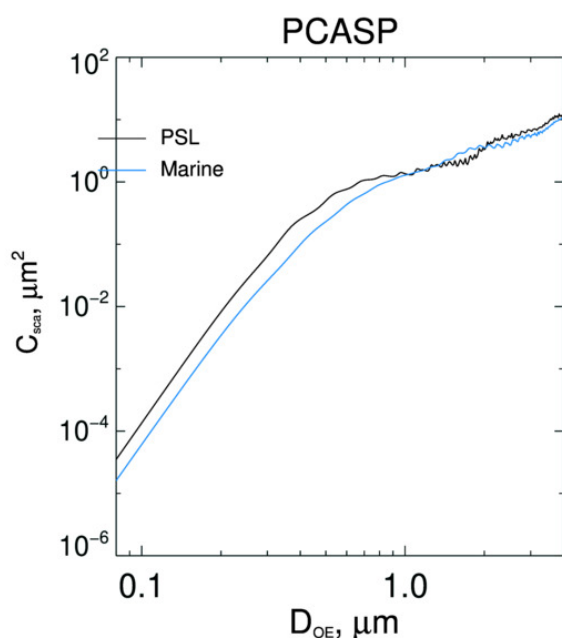
Figure 1. Scattering cross-section C_{\text{sca}} as a function of particle diameter calculated using Mie theory for the PCASP. The black line represents the C_{\text{sca}} for the calibration particles (PSL). The light-blue line represents the C_{\text{sca}} for marine aerosols ( m = 1.38 - 0.001i ). The small vertical gray lines represent the bin edges for the nominal calibration particles.
