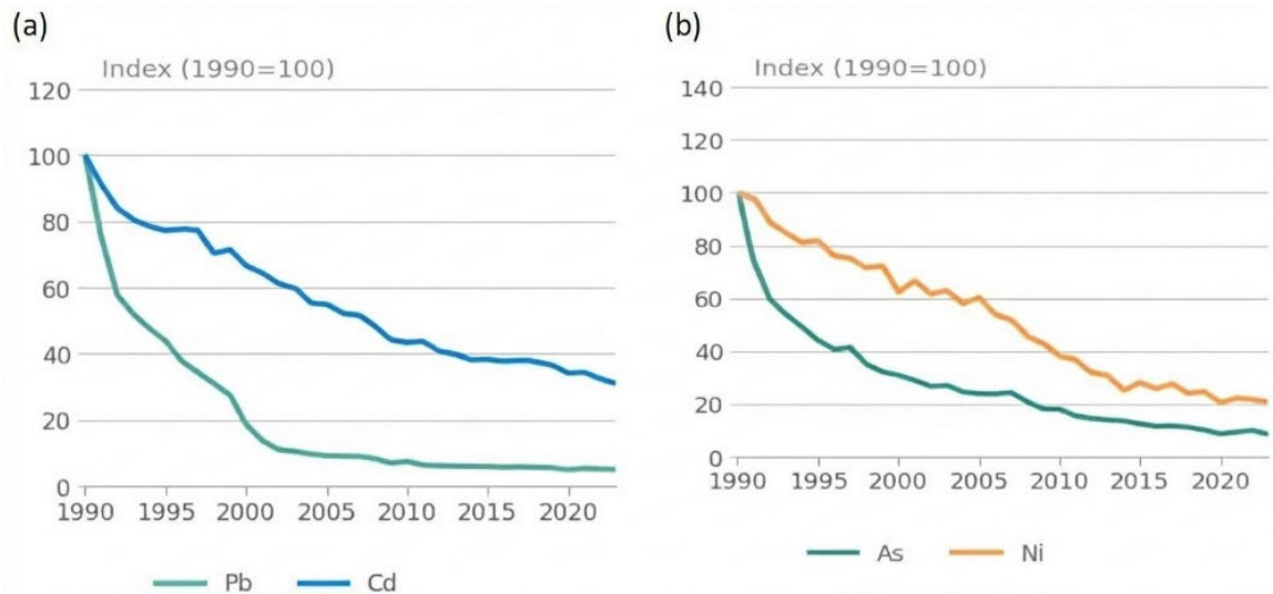
Figure S1: Indexed EU-27 emission trends for HMs. Reworked from (EEA, 2025).
