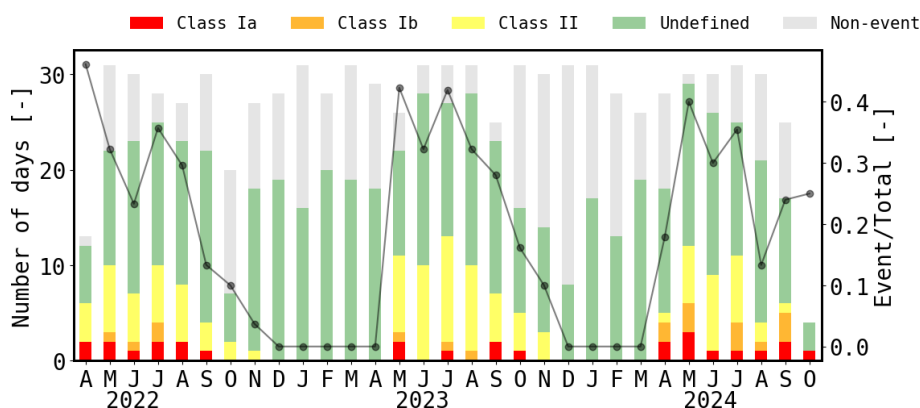
Figure 1. Number of days per month classified as either Class Ia (red), Class Ib (orange), Class II (yellow), undefined (green), or non-event (grey). The left-hand axis is the number of days classified based on the total number of valid measurement days (i.e. total). The right-hand side is the fraction of events (i.e. Class Ia, Ib, and II) over the total number of valid measurement days (i.e. Class Ia, Class Ib, Class II, undefined, and non-event). The fraction is given by event/total. Almost 3 years of Neutral cluster and Air Ion Spectrometer (NAIS) particle number size distribution data is classified using the Dal Maso et al. (2005) classification system.
