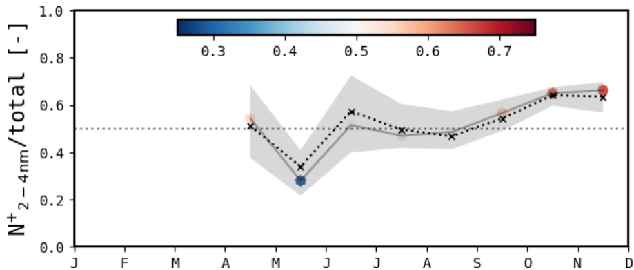
Figure 6. For all new particle formation (NPF) events the monthly ratio of the total number concentration of positively charged small intermediate ions (2–4 nm) over the total concentration of both positively and negatively charged small intermediate ions ( N_{2-4\text{ nm}}^+ / N_{2-4\text{ nm}}^- + N_{2-4\text{ nm}}^+ ). N_{2-4\text{ nm}}^- and N_{2-4\text{ nm}}^+ include only ion concentrations within the identified growing mode between 2 and 4 nm. The mean monthly N_{2-4\text{ nm}}^+ / \text{total} is presented as a cross, and the median is displayed by coloured circles, blue for an overall negative charge (ratio < 0.5) and red for an overall positive charge (ratio > 0.5). The grey shading displays the 25th–75th percentiles. The dashed black line represents an overall neutral charge of small intermediate ions. It should be noted that there may be some instrumental biases between the two polarities; however, the background concentrations (during no-event periods) display N_{2-4\text{ nm}}^- / N_{2-4\text{ nm}}^+ ratios close to unity, \sim 1.02 .
