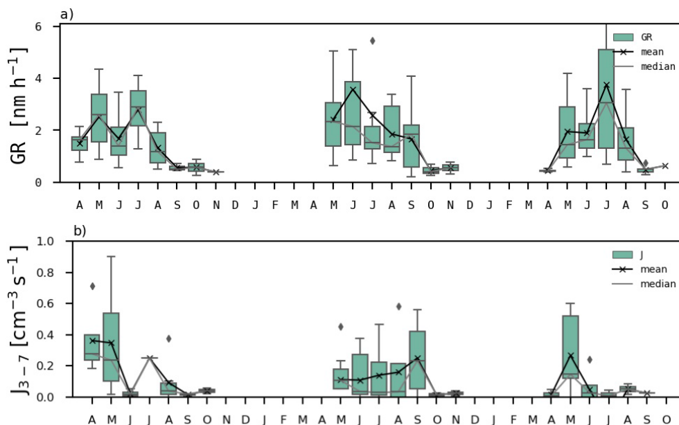
Figure 4. (a) The calculated growth rates (GRs) and (b) calculated median formation rates for particles between 3 and 7 nm ( J_{3-7} ) throughout the measurement period are represented by box whiskers, which display the monthly growth rate averages and include the median and 25th–75th percentiles. The green box whiskers refer to the average GRs/ J_{3-7} s from the start of the NPF until it stops growing. The black line with crosses represents the mean, and the grey lines join the median values. Diamonds represent outliers.
