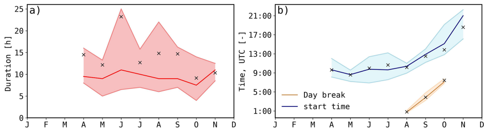
Figure 3. (a) Duration of the entire growth of newly formed particles from the first measurable size bin, i.e. 2.5 nm, to the largest size bin. (b) Average start time of the observed new particle formation (NPF) event. Monthly means displayed by crosses and medians by the red and blue lines, respectively, along with a shaded region representing the 25th and 75th percentiles. Time when the global horizontal irradiance (GHI) is greater than zero (i.e. daybreak) is displayed in orange. The average daybreak time for the months April until July is not applicable, since the sun is constantly above the horizon (as experienced by ZEP during the polar day). Time is given in terms of coordinated universal time (UTC). Note that a day break value for November to March is not applicable as these experience the polar night.
