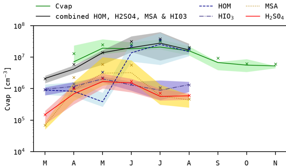
Figure 5. Estimated concentration of condensable vapours ( C_v ; solid green) compared with measured concentrations: the monthly means (crosses) and medians (thick line), along with the 25th and 75th percentiles (shaded region) for both C_v and Ny-Ålesund measurements. Arctic precursor vapours, namely sulfuric acid ( \text{H}_2\text{SO}_4 ; solid red), methanesulfonic acid (MSA; dotted gold), highly oxygenated molecules (HOMs; dashed dark blue), and iodic acid ( \text{HIO}_3 ; dash-dot purple), as well as combined values (grey) from Beck et al. (2021), are displayed. The estimated C_v measurements cover the years 2022 to 2024, whilst the Svalbard measurements from Beck et al. (2021) cover the period 22 March to 23 August 2017.
