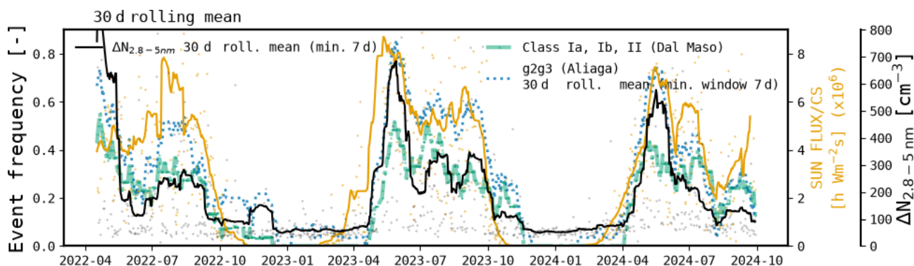
Figure 11. The solar insolation divided by the condensation sink (solar insolation/CS, SUN FLUX/CS) with a 30 d rolling mean is denoted by the orange line. The intensity parameter ( \Delta N_{2.8-5 \text{ nm}} ) is shown in black. The dash-dotted green and dotted blue lines represent the rolling averages of the NPF daily event frequencies using the Dal Maso et al. (2005) and Aliaga et al. (2023) classification schemes, respectively. The green and blue curves are displayed to be able to compare to the orange line, the proxy for NPF activity, i.e. the balance between sources and sinks.
