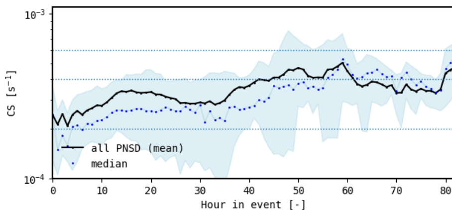
Figure 13. The calculated condensation sink (CS) during NPF events. It should be noted that the average NPF typically lasts for 10 h; however, in some cases events can persist for days until the newly formed mode is removed via wet scavenging or advected away from ZEP. The black line is the mean, and the blue is the median. The blue shaded region represents the 25th–75th percentiles. The dashed blue lines display CS values of 0.1, 0.2, and 0.4 \times 10^{-3} \text{ s}^{-1} and are there to guide the reader.
