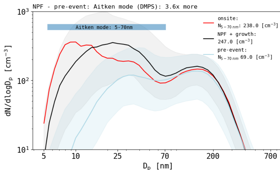
Figure 16. The particle number size distributions (DMPS) for periods before the NPF events (1–2 h before event started) (pre-event, light blue), during NPF and growth (black), and during on-site nucleation (production of 2–4 nm particles, red, on-site formation).
