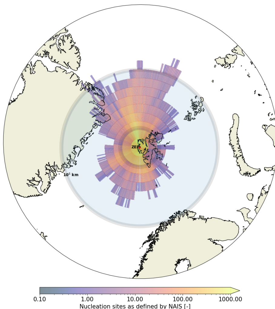
Figure 7. Total number of estimated nucleation sites per grid cell. The unit is based on the number of back trajectories initialised and does not reflect a physical value. Sites of nucleation for Class Ia, Ib, and II events are estimated by using HYSPLIT to trace the likely origin of particles produced during NPF events and initialising the back trajectories based on the duration of the NPF event (see Sect. 2.4.4).
