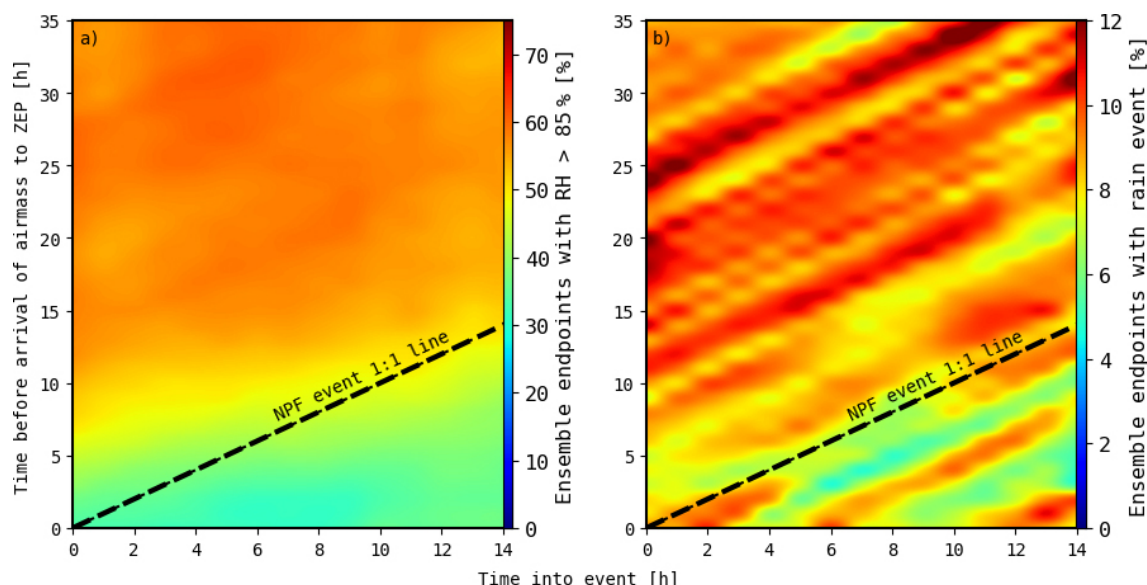
Figure 14. Air mass history for (a) percentage of back trajectory endpoints within an ensemble with a relative humidity above 85 and (b) percentage of endpoints within an ensemble which experienced a rainfall event (i.e. rainfall > 0 mm). The y axis is the number of hours backwards before the air masses arrive at ZEP, while the x axis is the number of hours into the event; e.g. if one event started at 06:00 and another at 09:00, their start times would both be 00:00. The black line is a 1 : 1 line which represents the start of the NPF event such that the grid points towards the top left represent endpoints prior to the NPF event, whilst grid points towards the bottom right represent endpoints during the NPF event. The x axis has been sliced based on the typical duration of events (most events are < 14 h). This figure consists of the air mass history of Class Ia and Ib NPF events.
