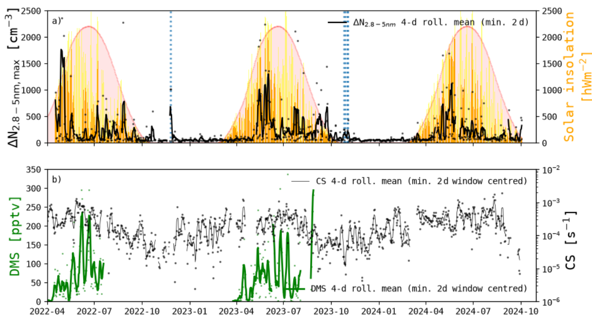
Figure 2. Time series of (a) the NPF intensity parameter ( \Delta N_{\max,2.8-5} ; black dots), defined as the daily maximum particle number concentration between 2.8 and 5 nm. The black line shows the centred 4 d running mean. Orange bars indicate daily solar insolation accumulated over the preceding 6 h for air masses arriving at ZEP within the mixed layer (Sect. 2.4.1); faint yellow bars show the same for all air masses. The red shaded region is there for comparison to the yellow and orange bars and represents 6 times the average hourly clear-sky global horizontal irradiance (GHI) at ZEP. (b) Valid DMS measurements (green) and the condensation sink (CS; black dots, daily means) with its centred 4 d running mean (black line). Dashed blue lines indicate polar-night periods.
