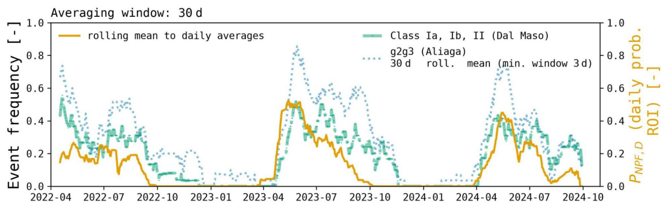
Figure 10. The orange line is P_{\text{NPF},D} , the estimated daily likelihood of measurements occurring in the region of interest (ROI). The ROI is based on the relation between CS and 6 h solar accumulation and is defined in Fig. 8. The dash-dotted green and dotted blue lines represent the rolling averages of the NPF daily event frequencies using the Dal Maso et al. (2005) and Aliaga et al. (2023) classification, respectively. The green and blue curves are present here to be able to compare to P_{\text{NPF},D} .
