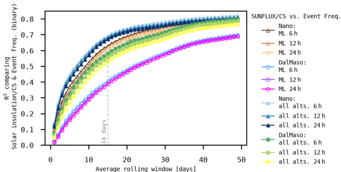
Figure 12. Correlation between the event frequency (defined using either the Dal Maso (circles) or nano-ranking (triangles) classification method) and the ratio of the accumulated solar insolation and CS (SUNFLUX/CS) with a rolling average applied. The coefficient of determination ( R^2 ) is a function of the rolling window size (i.e. number of days). The first 6, 12, and 24 h of the back trajectories are selected (in different shades). The curve labelled ML (empty symbols) represents back trajectories that traversed only through the mixed layer, while the curves labelled “all alts.” (whole symbols) represent back trajectories at all altitudes. Dashed grey line at 14 d to indicate plateauing of R^2 .
