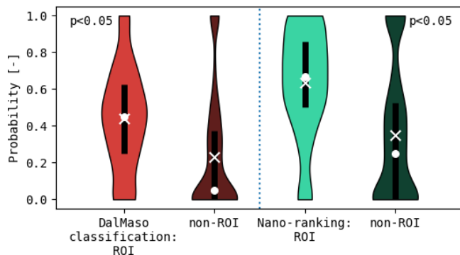
Figure 9. Violin plots representing the distribution of the probabilities as defined by the normalisation plot (see Fig. 8). The red violins on the left-hand side represent the probability distributions related to the Dal Maso et al. (2005) classification, and the green violins on the right-hand side represent the probability distributions according to the nano-ranking approach.
