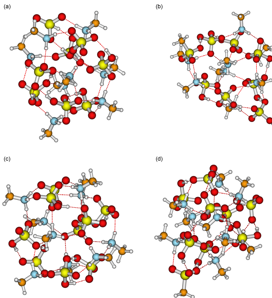
Figure 2. Comparison of pure and mixed-acid clusters for the MA system. (a) (\text{SA})_8(\text{MA})_8 , (b) (\text{MSA})_1(\text{SA})_7(\text{MA})_8 , (c) (\text{SA})_9(\text{MA})_9 , (d) (\text{MSA})_1(\text{SA})_8(\text{MA})_9 .
