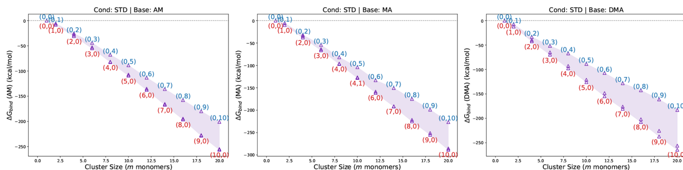
Figure 1. Binding Gibbs free energies ( \Delta G_{\text{bind}} ) at the B97-3c level of theory under standard conditions (STD) for clusters containing SA, MSA, and bases (AM, MA, DMA). The shaded region represents the range between minimum and maximum values for each cluster size, while annotations indicate the acid composition (SA, MSA).
