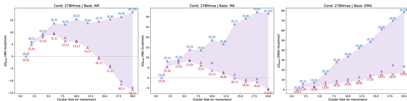
Figure 5. Binding Gibbs free energies ( \Delta G_{\text{bind}} ) at the B97-3c level of theory at 278.15 K under high-MSA-concentration conditions (278Hmsa), with [\text{SA}] = 10^6 and [\text{MSA}] = 10^8 molec. \text{cm}^{-3} . Base concentrations are fixed at AM = 10 ppb and amines (MA, DMA) = 5 ppt.
