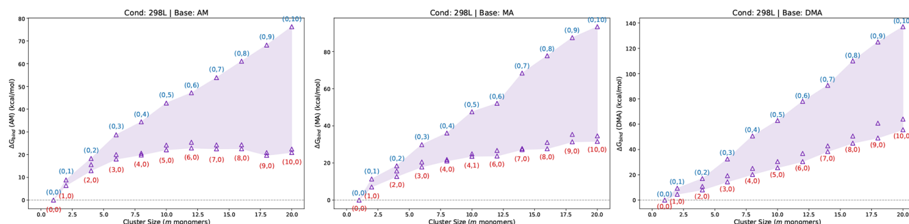
Figure 3. Binding Gibbs free energies ( \Delta G_{\text{bind}} ) at the B97-3c level of theory at 298.15 K under low-concentration conditions (298L), with [\text{SA}] = [\text{MSA}] = 10^6 \text{ molec. cm}^{-3} . Base concentrations are fixed at AM = 10 ppb and amines (MA, DMA) = 5 ppt.
