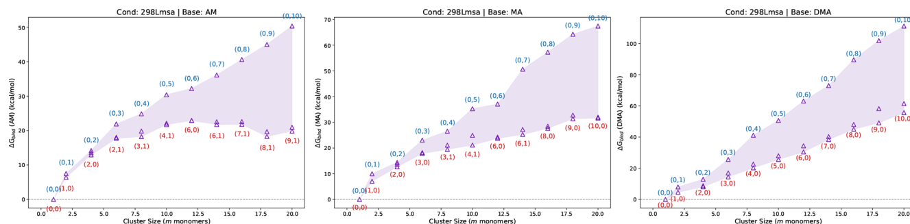
Figure 4. Binding Gibbs free energies ( \Delta G_{\text{bind}} ) at the B97-3c level of theory at 298.15 K under low-SA- and high-MSA-concentration conditions (298Lmsa), with [\text{SA}] = 10^6 and [\text{MSA}] = 10^8 \text{ molec. cm}^{-3} . Base concentrations are fixed at AM = 10 ppb and amines (MA, DMA) = 5 ppt.
