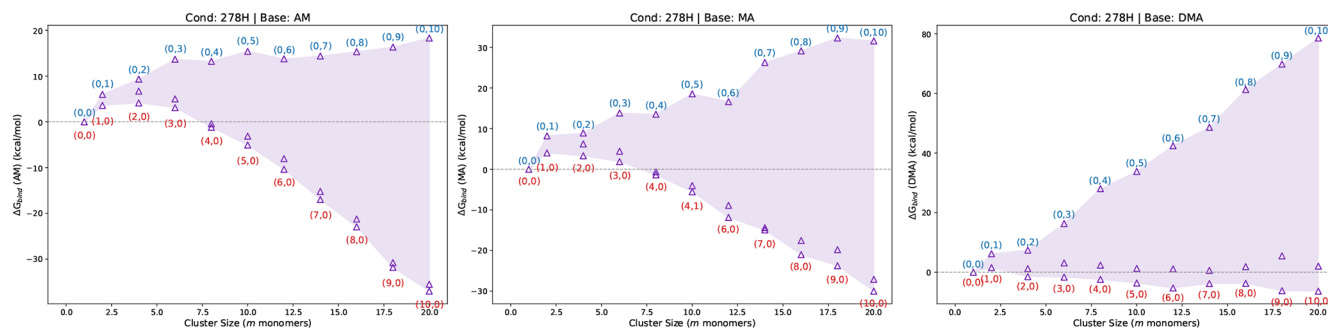
Figure 6. Binding Gibbs free energies ( \Delta G_{\text{bind}} ) at the B97-3c level of theory at 278.15 K under high-concentration conditions (278H), with [\text{SA}] = [\text{MSA}] = 10^8 molec. \text{cm}^{-3} . Base concentrations are fixed at AM = 10 ppb and amines (MA, DMA) = 5 ppt.
