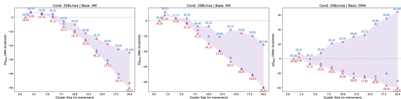
Figure 7. Binding Gibbs free energies ( \Delta G_{\text{bind}} ) at the B97-3c level of theory at 258.15 K under MSA-rich conditions (258Lmsa), with [\text{SA}] = 10^6 and [\text{MSA}] = 10^9 molec. \text{cm}^{-3} . Base concentrations are fixed at AM = 10 ppb and amines (MA, DMA) = 5 ppt.
