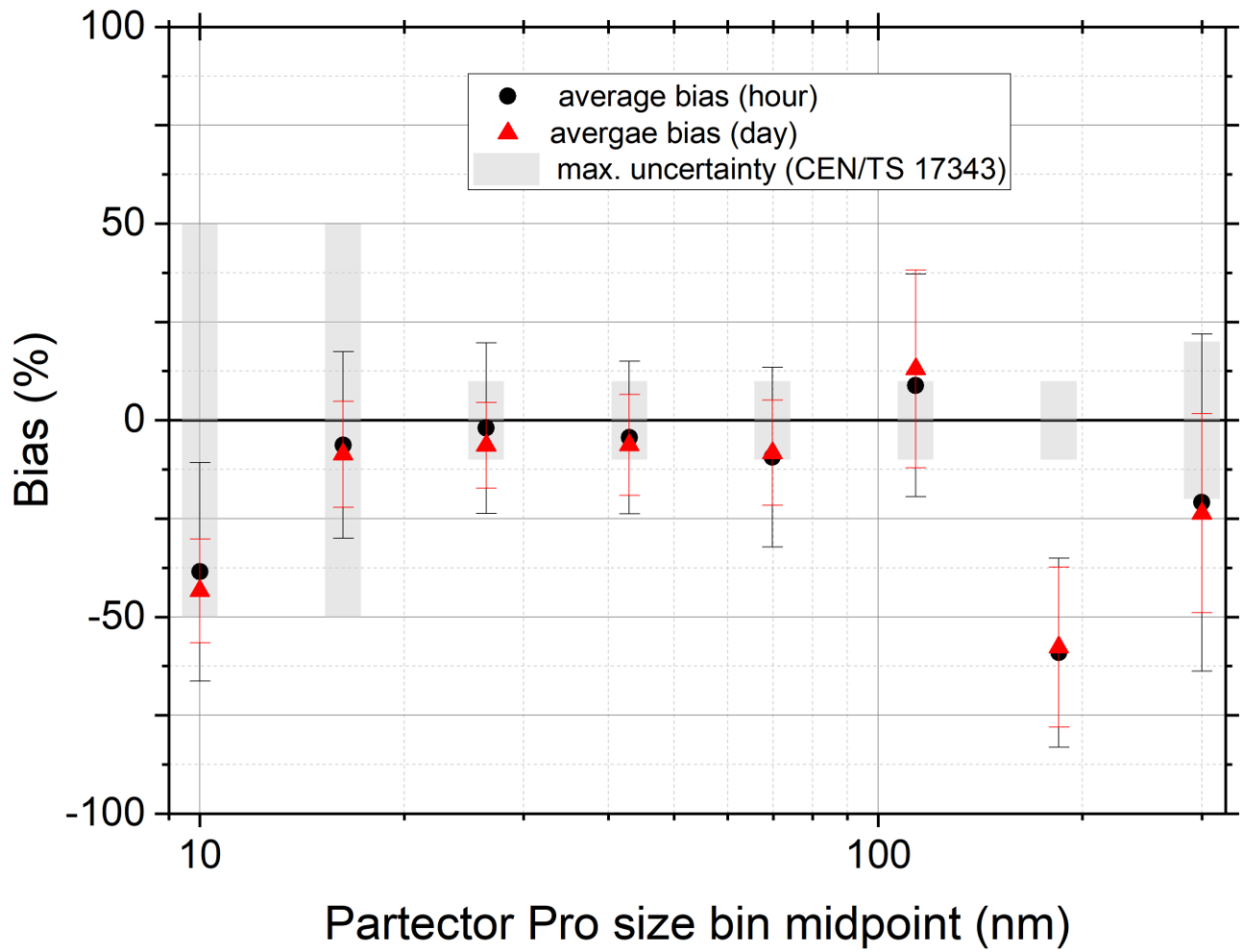
Figure 5: Bias of the number concentration per Partector Pro size bin as hourly (black circle) and daily (red triangle) averages; error bars display the standard deviations
