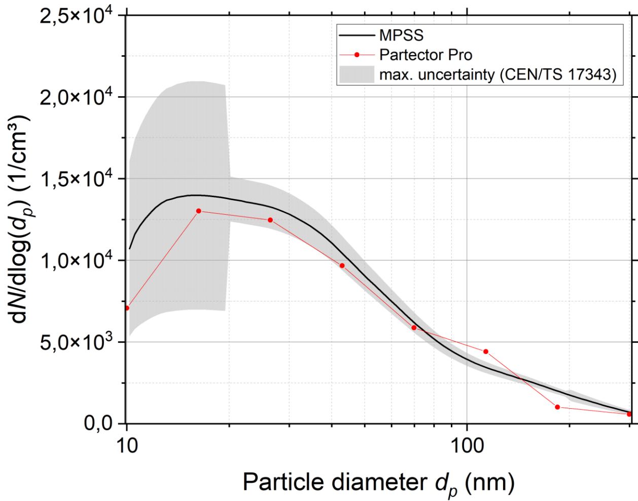
560 Figure 4: Mean particle size distribution during the measurement period, measured with the MPSS and Partector Pro; grey shaded area illustrates the allowed uncertainty range according to CEN/TS 17343
