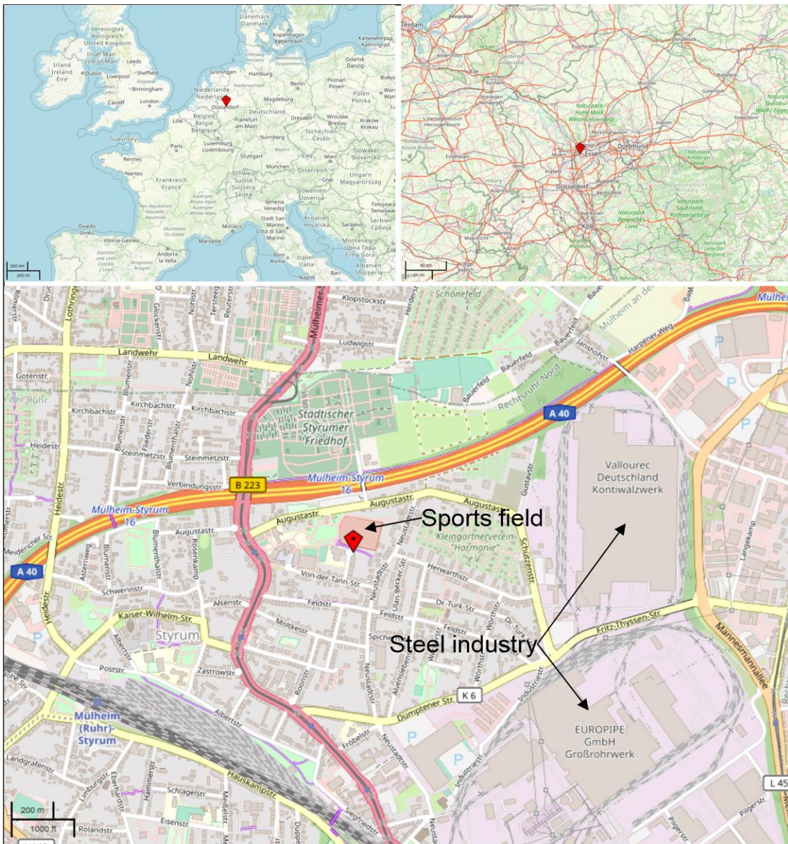
Figure 1: Location (red marker) in central Europe (top left), western Germany (top right) and direct vicinity (bottom) of the measurement location in Mülheim-Styrum (map © OpenStreetMap contributors 2023. Distributed under the Open Data Commons Open Database License (ODbL) v1.0.)
