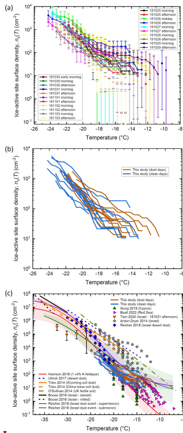
Figure 6: Plots showing the ice-active site surface density, n_s(T) for INPs in Israel. (a) Background-subtracted n_s(T) spectra for 3 h filter samples. Dates are given in the YYYYMMDD format. (b) The 3 h filter sample data separated into dust events (brown) and clean days (blue). (c) Comparison of n_s(T) values to relevant literature, including n_s(T) data from Israel and the East Mediterranean region (Ardon-Dryer and Levin, 2014; Beall et al., 2022; Gong et al., 2019; Reicher et al., 2019; Reicher et al., 2018; Tarn et al., 2020). Several parameterisations for mineral dust are provided, including those for surface samples from arid locations around the world (Ullrich et al., 2017), sieved and milled surface samples from Israel (Boose et al., 2016), supermicron and submicron particles in desert dust storms (Reicher et al., 2019), the Harrison parameterisation for K-feldspar assuming K-feldspar comprised around 1 wt% of airborne mineral dust (Harrison et al., 2019). Parameterisations are provided for fertile soils (O'Sullivan et al., 2014) and agricultural soils (Tobo et al., 2014).
