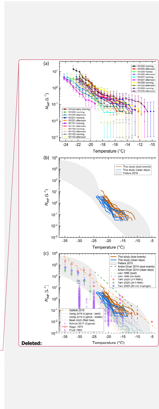
445 Figure 1: Plots showing ice-nucleating particle (INP) concentrations ( N_{INP} ) in Israel. (a) Background-subtracted INP concentration spectra for samples collected for 3 h onto filters from 25 th October–4 th November 2018. The temperature error is estimated to be 0.4
