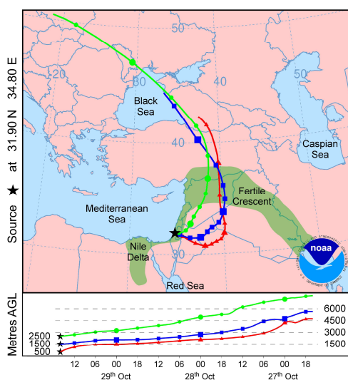
Figure 3: Air mass back trajectory (72 h duration) for the 29 th October 2018 (E D2 ), obtained using NOAA’s HYSPLIT tool, showing three arrival heights at the sampling site: 500 m (red), 1,500 m (blue), and 2,500 m (green) above ground level (AGL). The approximate location of the ancient Fertile Crescent region is shown in dark green. The black star represents the sampling site.
