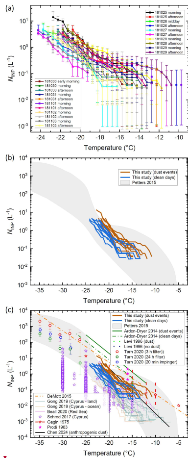
445 Figure 1: Plots showing ice-nucleating particle (INP) concentrations ( N_{INP} ) in Israel. (a) Background-subtracted INP concentration spectra for samples collected for 3 h onto filters from 25 th October–4 th November 2018. The temperature error is estimated to be 0.4
