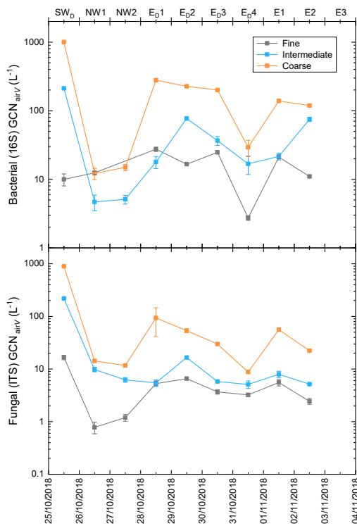
655 Figure 5: Plots showing size-resolved biological aerosol particle concentrations, in terms of gene copy number (GCN) per litre of air, for (a) bacteria, analysed using 16S ribosomal RNA, and (b) fungi, using the ribosomal internal transcribed spacer (ITS) region. Particle size ranges were stratified into: coarse (3 \mu\text{m} – 18 \mu\text{m} ), intermediate (0.8 \mu\text{m} – 3 \mu\text{m} ) and fine (<1.3 \mu\text{m} ).
