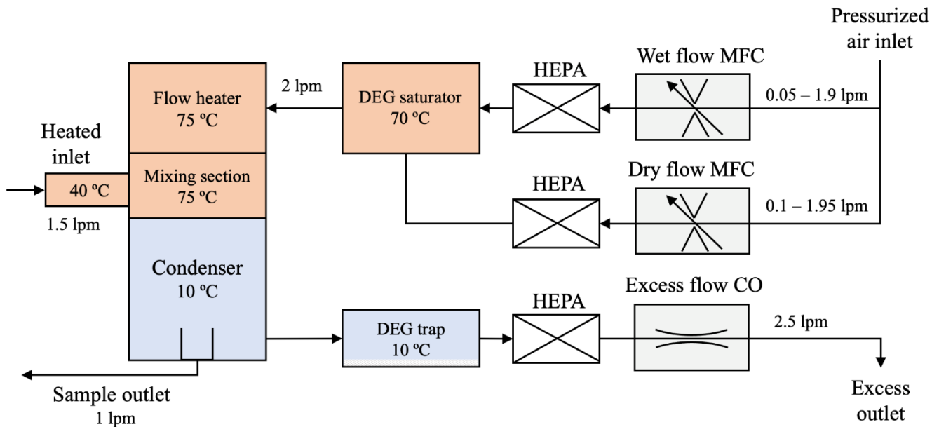
Figure 1. The flow diagram of the prototype PSM 2.0.
