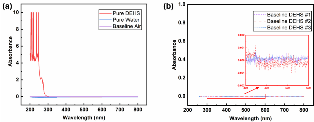
Figure 6: UV-Vis spectra of water and DEHS when using air as the baseline and (b) Baselines obtained from measurements with different batches of DEHS.
