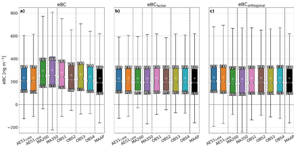
Figure 5. Calibration methods. Panel a) is data without calibration. Panel b) is data calibrated by the F -factor calculated by comparing 1 st intercomparison data means. Panel c) is data calibrated with the orthogonal fit equations. In the boxplots the middle line shows the median, “+” shows mean, top of box 75 th percentile, bottom of the box 25 th percentile and top and bottom whisker the last points within 1.5 times the interquartile range. The values are the mean (top) and median (bottom).
