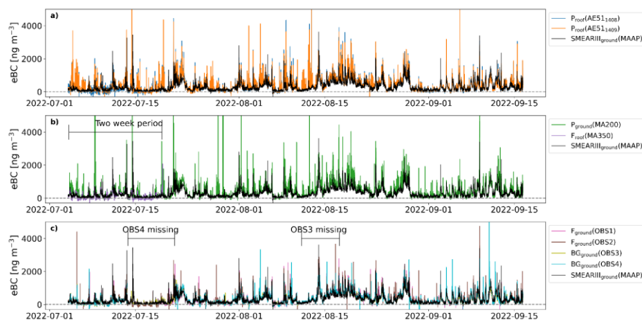
Figure 7. Time series of eBC for the deployment period for a) AE51 sensors, b) MA-series sensors, and c) Observair (OBS) sensors. Each panel has also the SMEARIII_{ground} measurement by the multi-angle absorption photometer (MAAP) reported. Data are in 5-min averages. The two week period, when all the instruments were operational is marked in panel b) and the periods when OBS3&4 sensors were malfunctioning are marked in panel c).
