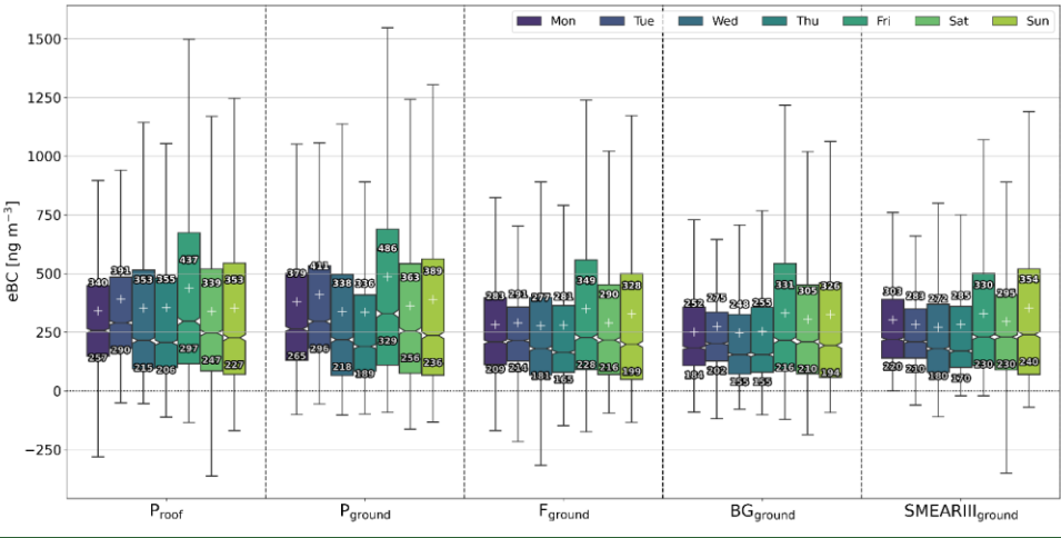
Figure 10. Daily eBC concentrations for different sensors. In the boxplot every sensor has 7 boxes going left to right as Mon–Sun (indicated with different colors). The explanation for the boxes is the same as in Fig. 5.
