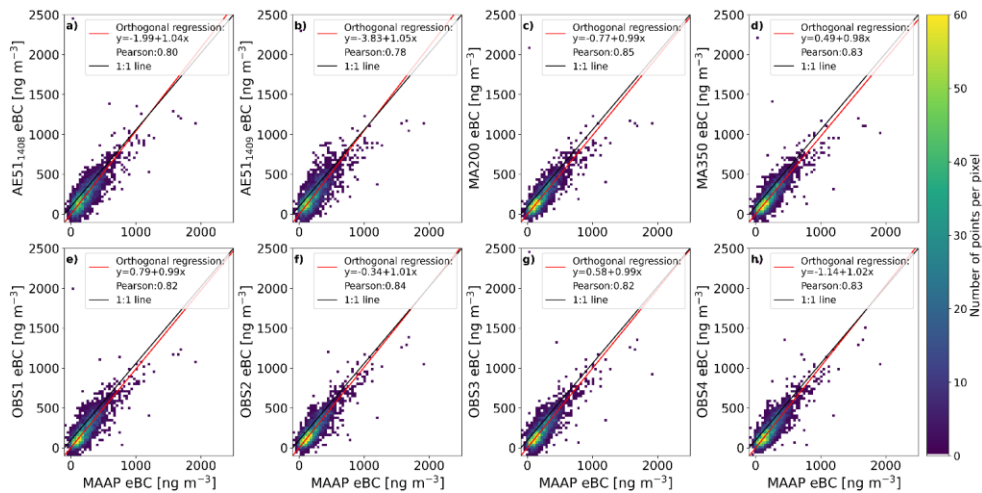
Figure 6. Correlation and orthogonal regression line fits after calibrating with the orthogonal regression equations see presented in Fig. 3 and Table 4. Data are from 1 st intercomparisons 26.5–6.6.2022 as 5-min averages.
