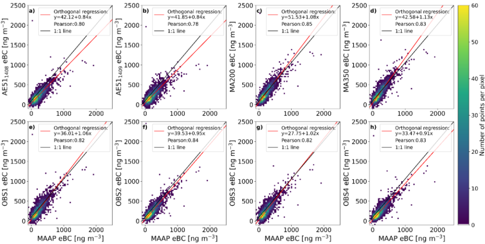
Figure 3. Scatter density plot of the correlation between the eBC sensors and the reference instrument MAAP. Data are from 1 st intercomparisons 26.5.—6.6.2022 as 5-minute averages.
