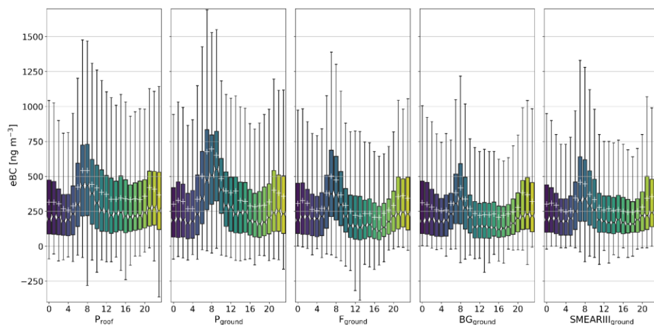
Figure 11. Hourly variation of eBC concentrations. In the boxplot every sensor has 24 boxes going from 00An hourly-23 where the box describes the hour of the day. The explanation for the boxes is the same as in Fig. 5.
