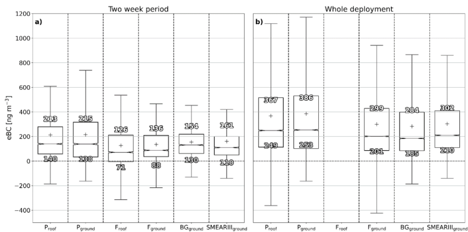
Figure 8. Boxplots of eBC concentration from the whole deployment period. Panel a) data are only from the first 15 days (4.7–19.7) of the deployment when all the instruments were operational; and b) data are from the whole deployment phase (74 d). The explanation for the boxes is the same as in Fig. 5.
