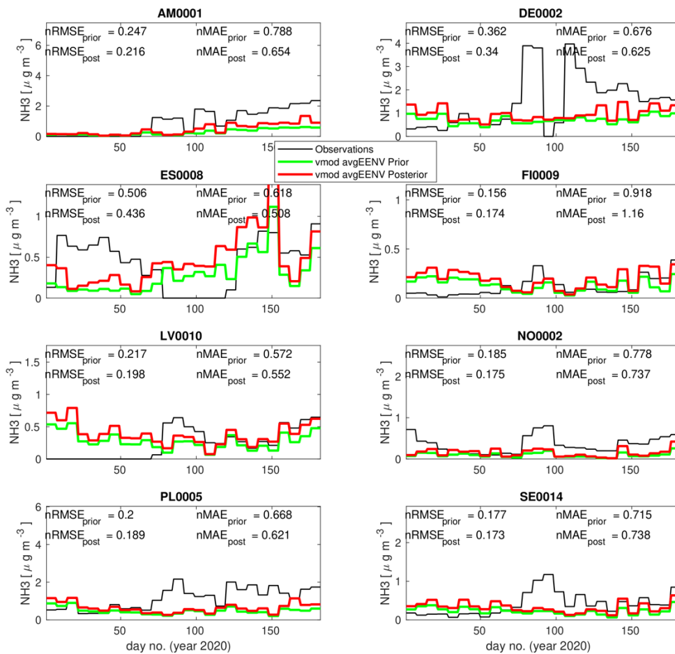
Figure S 4. Timeseries of prior and posterior ammonia against observations from eight EMEP sites. In most cases better statistics were obtained with respect to RMSEs and MAEs.
