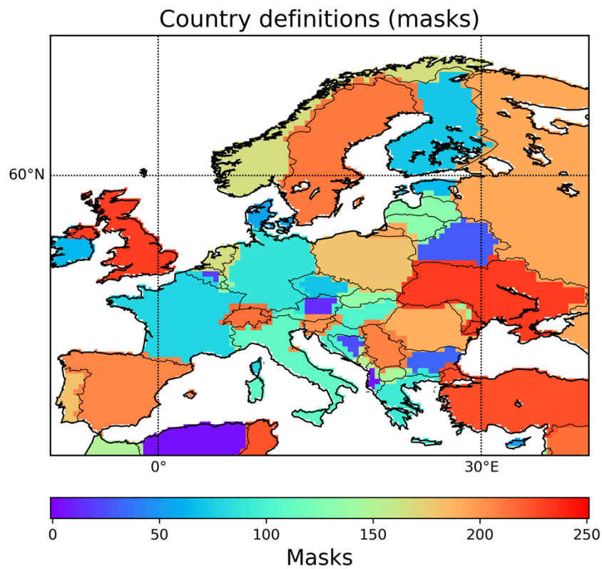
Figure S 5. Country masks used to calculate emissions of ammonia over different European countries, namely Austria, Belgium, Denmark, Finland, France, Germany, Greece, Iceland, Ireland, Italy, Luxembourg, Netherlands, Norway, Portugal, Spain, Sweden, Switzerland, Turkey, United Kingdom, Albania, Belarus, Bosnia and Herzegovina, Bulgaria, Croatia, Cyprus, Czechia, Estonia, Hungary, Latvia, Lithuania, Malta, Poland, Republic of Moldova, Romania, Slovakia, Slovenia, North Macedonia, Ukraine, Serbia (Russian Federation was excluded from the study).
