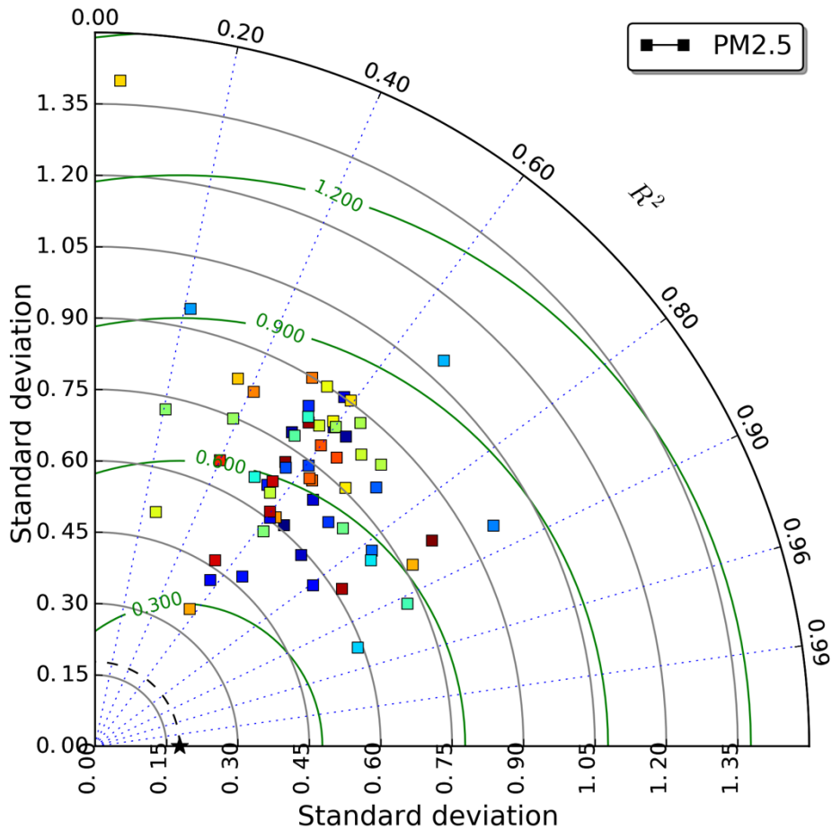
Figure S 6. Modelled concentrations of PM 2.5 against ground-based observations from EMEP stations (79 sites) for January to June 2020 presented in a Taylor diagram. The diagram shows the Pearson's correlation coefficient (gauging similarity in pattern between the modelled and observed concentrations) that is related to the azimuthal angle (blue contours); the standard deviation of modelled concentrations of ammonia is proportional to the radial distance from the origin (black contours) and the centered normalized RMSE of modelled concentrations is proportional to the distance from the reference standard deviation (green contours).
