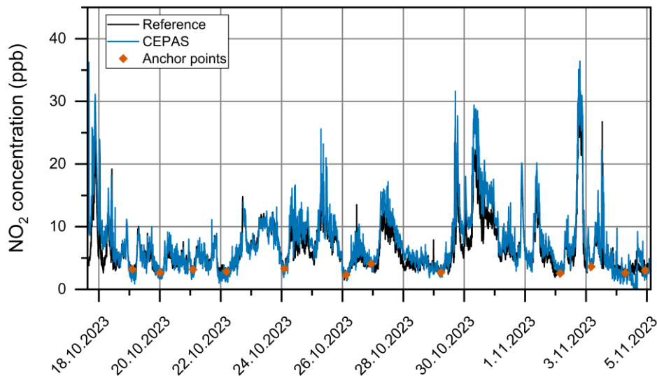
Figure 6: NO 2 concentration calculated from the CEPAS background signals. NO 2 concentration measured with a chemiluminescence instrument is shown for reference. To account for background drifting, the NO 2 concentration measured with the two instruments was matched at the marked anchor points. Averaging time for both data is 5 min.
