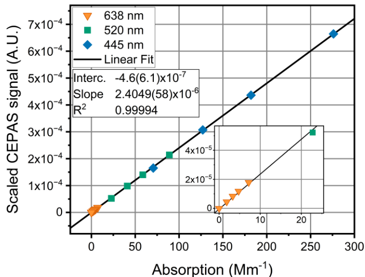
Figure A1: CEPAS signal, scaled by optical power and frequency response at each channel, as a function of the NO 2 absorption. The scaling allows applying all the calibration data measured at the different wavelengths to the same calibration fit. The NO 2 absorption is calculated for the different wavelengths from literature NO 2 absorption cross section, at each NO 2 concentration steps. Values scaled from the red, green and blue channels are shown with different coloured symbols.
