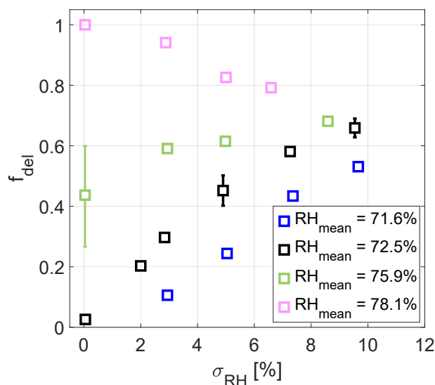
Figure 4. Deliquesced particle fraction f_{del} as a function of the standard deviation of the RH distribution \sigma_{RH} . The width of the symbols represents the range of uncertainty of \sigma_{RH} based on the LES results. The shown error bars originate from repeated measurements (three to five times) giving the minimal and maximal obtained f_{del} , respectively.
