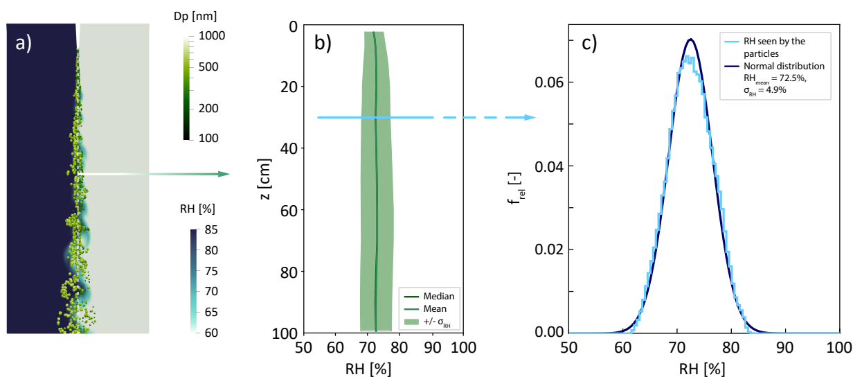
Figure 2. a) A snapshot of the particle simulation with the fluctuating RH field in the background (flow direction from top to bottom). It depicts the scenario of RH_A = 60\% (right side) and RH_B = 85\% (left side) resulting in a mean RH of 72.5% along the center line (dashed white line). Note that only 10% of the particles are depicted. The particles are colored and sized (not to scale) according to their diameter. b) The obtained temporal median RH, mean RH, and RH fluctuations in terms of \pm \sigma_{RH} plotted along the center line as a function of the distance z to the aerosol inlet of the measurement section. Note that the pre-humidified aerosol is injected (case(ii): RH = 70.2\% at 15^\circ\text{C} ). c) The normalized frequency of the RH experienced by the particles. The distribution has a Gaussian shape as evidenced by the normal distribution with RH_{mean} = 72.5\% and \sigma_{RH} = 4.9\% .
