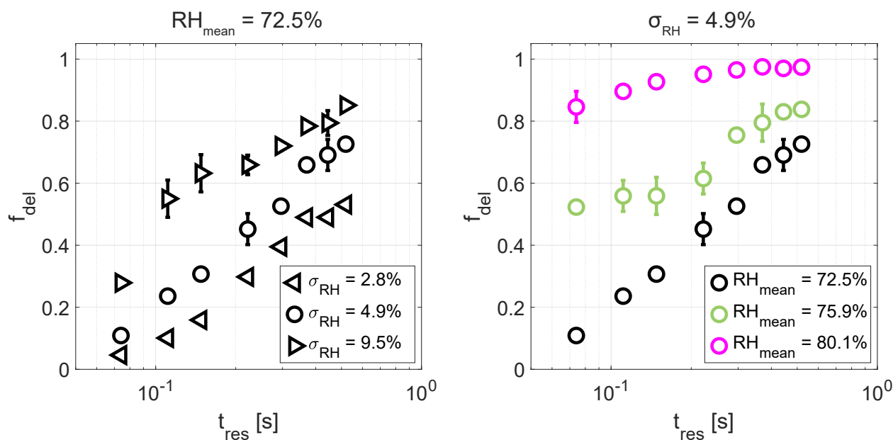
Figure 6. Deliquesced particle fraction f_{del} as a function of particle residence time t_{res} . Left figure: RH_{mean} was set to 72.5% and \sigma_{RH} was varied. Right figure: \sigma_{RH} was set to 4.9% and RH_{mean} was varied.
