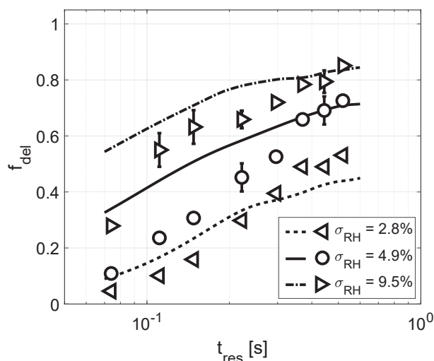
Figure B1. Measured (symbols) and simulated (lines) deliquesced particle fraction f_{\text{del}} as a function of particle residence time t_{\text{res}} for RH_{\text{mean}} = 72.5\% .
