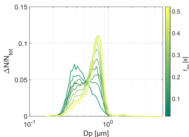
Figure 5. Normalized particle number size distributions determined experimentally for \text{RH}_{\text{mean}} = 75.9\% and \sigma_{\text{RH}} = 4.9\% , but for different residence times t_{\text{res}} inside the measurement section. The colors of the different number distributions correspond to the colormap on the right-hand side of the plot denoting t_{\text{res}} .
