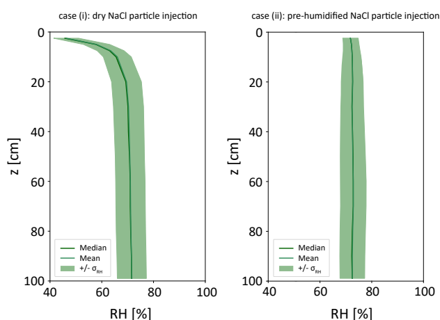
Figure A1. LES results for the scenario of RH_A = 60\% and RH_B = 85\% which results in a mean RH of 72.5% along the center region (i.e., the main mixing zone). The obtained median RH, mean RH and RH fluctuations in terms of \pm\sigma_{RH} are plotted for the center region as a function of the distance z to the aerosol inlet of the measurement section for two different types of particle injection. Left figure: Injection of dry aerosol (case (i): RH \leq 5\% at 15^\circ\text{C} ). Right figure: Injection of pre-humidified aerosol (case(ii): RH = 70.2\% at 15^\circ\text{C} ).
