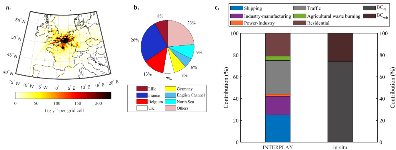
Figure 2: (a) Spatial contribution of BC to ATOLL in Gg\ y^{-1} per grid cell and its (b) relative contribution by region/country, note that France does not include Lille's contribution; c) sectorial distributions according to INTERPLAY and in-situ via the aethalometer model. Results over the period Dec 2016 – Dec 2019.
