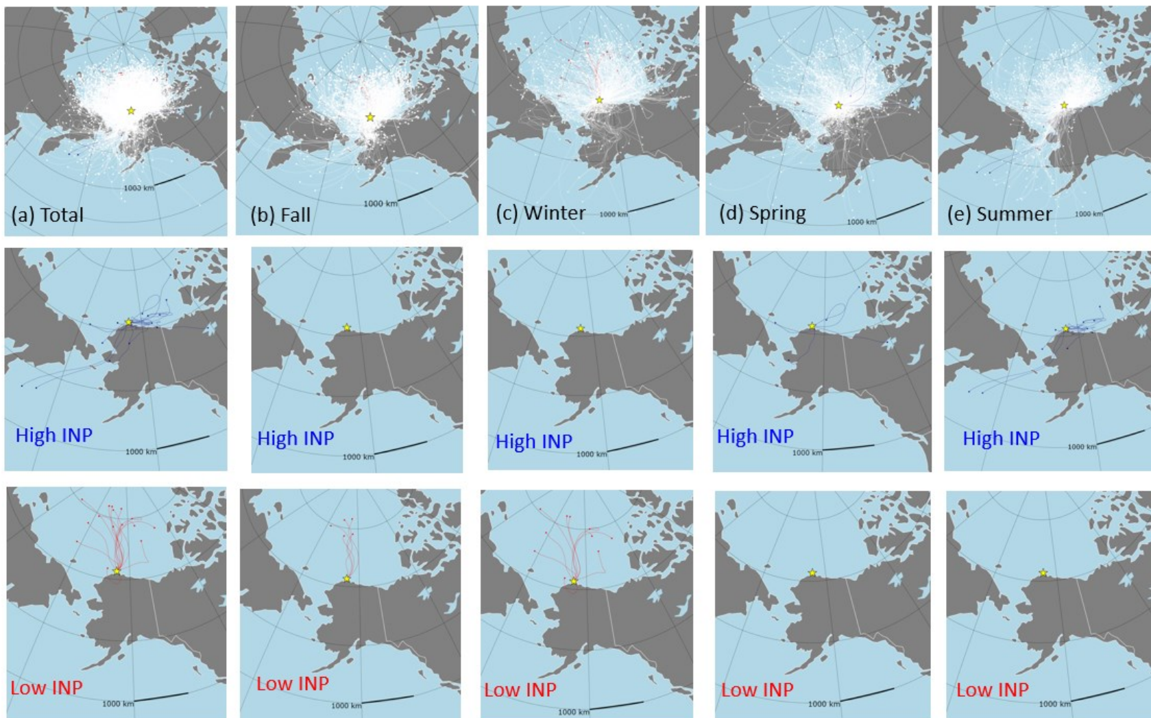
Figure S8. Air mass origins and back trajectories at the inlet height from BRW; all trajectories in October 2021 – December 2023. The air mass trajectories during high- and low-INP episodes are shown in blue and red colors. This figure represents the data selected with a low – high threshold of the 25 th – 75 th percentile based on n_s , at -30 , -25 , and -20 °C (below or above at ‘all’ temps). Figure S8a represents the overall data. Panels (b) – (e) are seasonal breakdowns of the ‘clean’ fall, winter, spring, and summer, respectively.
