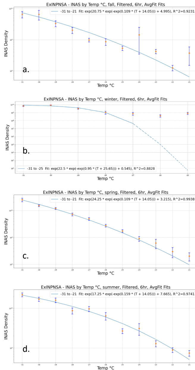
185 Figure S5. Seasonal n_s(T) parameterizations that fit the median values of the log-normal n_s(T) distribution as a function of freezing temperatures based on the clean data; fall (a), winter (b), spring (c), and summer (d).
