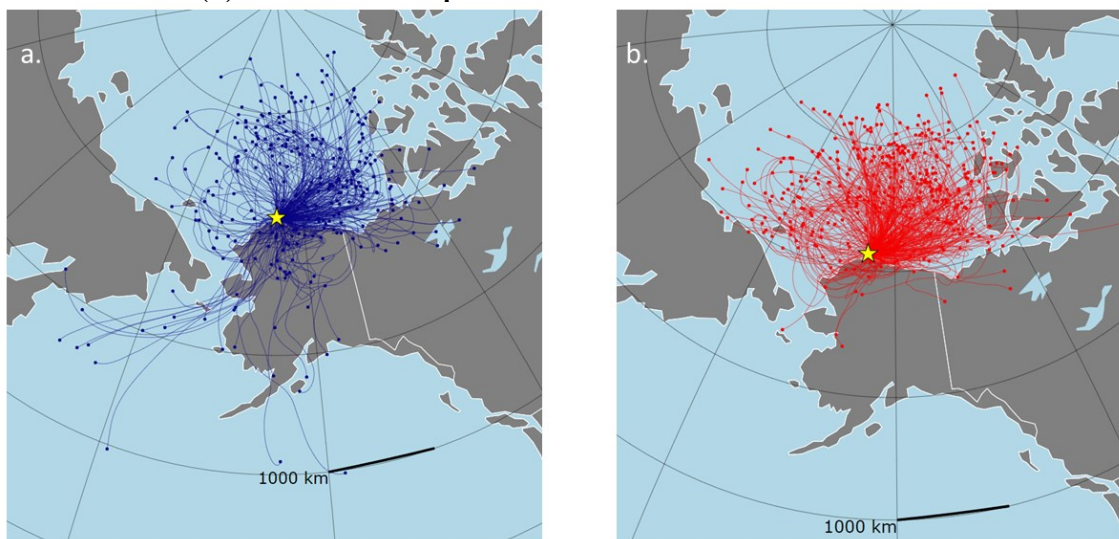
200 Figure S7. Air mass origins and back trajectories at the inlet height from BRW (yellow star). The air mass trajectories during high- and low-INP episodes are shown in blue and red colors. Panel (a) represents the data selected with a low – high threshold of the 25 th – 75 th percentile based on n_s , at any -30 , -25 , and -20 °C (below or above at ‘any’ temps). Panel (b) represents the data selected with a low – high INP threshold of the 25 th – 75 th percentile based on n_s(T) at any selected temperatures. 205
