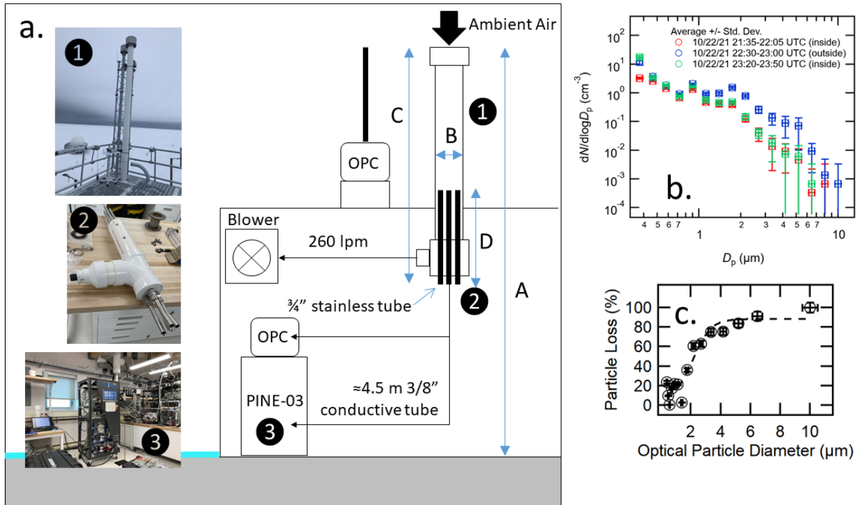
50 Figure S1: Panel (a) shows an experimental schematic of the particle loss test through the PVC stack inlet at the BRW site (A = 12 m; B = 0.1 m; C = 7.6 m; D = 0.9 m). Panels (b) and (c) show the particle size distributions measured inside and outside the observatory and particle loss through the inlet as a function of particle diameter. Each data point is shown \pm a 5% size uncertainty on the x-axis and \pm the standard deviation of three measurements on the y-axis (20-second time average for each data point).
