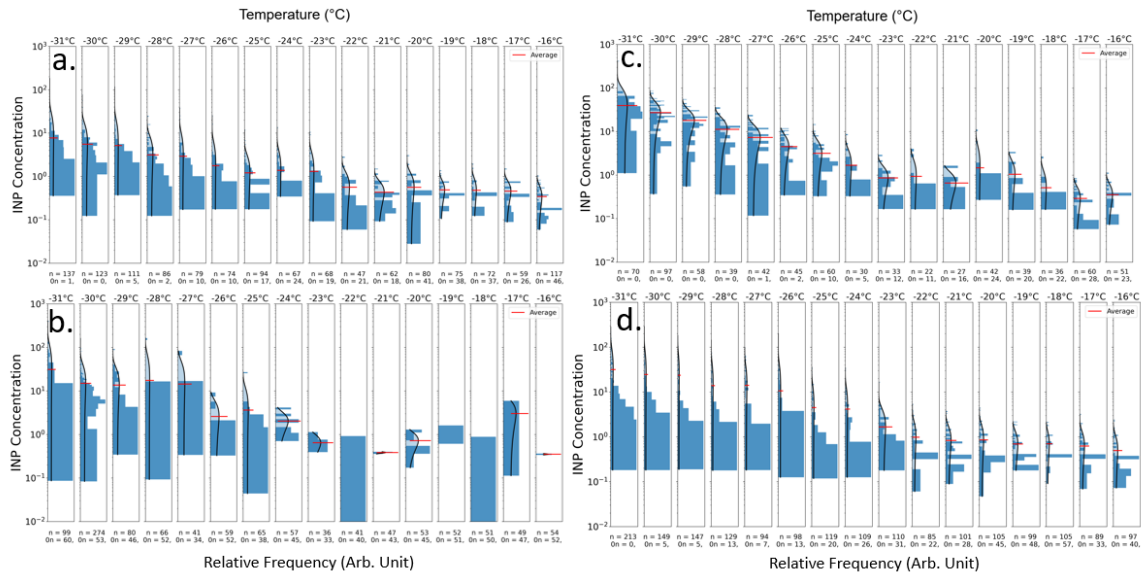
Figure S2. Histogram of the seasonally resolved m_{\text{INP}}(T) Gaussian distribution with a degree temperature bin for a statistically validated freezing temperature range ( -16 to -31 °C). Panels (a) – (d) are seasonal breakdowns of the clean fall, winter, spring, and summer, respectively. Individual data densities, zero INP counts, and relative frequencies (Arbitrary Unit) for each degree are shown at the bottom of each panel. Red horizontal lines in each relative frequency distribution sub-panel represent the average. Figure 6a in the main manuscript represents the overall data.
