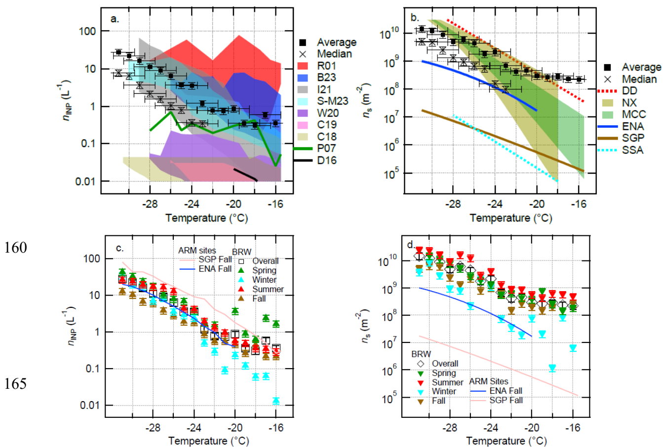
170 Figure S4. Box plot of the PINE-03 based n_{\text{INP}}(T) and n_s(T) spectra with a degree temperature bin for a statistically validated freezing temperature range at BRW (a – b; –16 to –31 °C). The ‘all’ data were used to generate this figure. Individual data points display average (black solid symbol) and median (black open symbol) in Panel a. The color-shaded area in panel (a) shows the maximum and minimum n_{\text{INP}}(T) measured by previous INP studies at or in the proximity of BRW (see Table A1 and Sect. 1 for references). The reference n_s(T) spectra in panels (b) are adopted from W24 (Wilbourn et al., 2024 and references therein) for SGP, ENA, Desert Dust, Sea Spray Aerosol, illite NX, and microcrystalline cellulose. Panels (c) and (d) are seasonal breakdowns of the average data presented in Panels a and b, respectively. The vertical bars are adopted from W24. Note: the temperature uncertainty of PINE-03 is \pm 1.5 °C. 175
