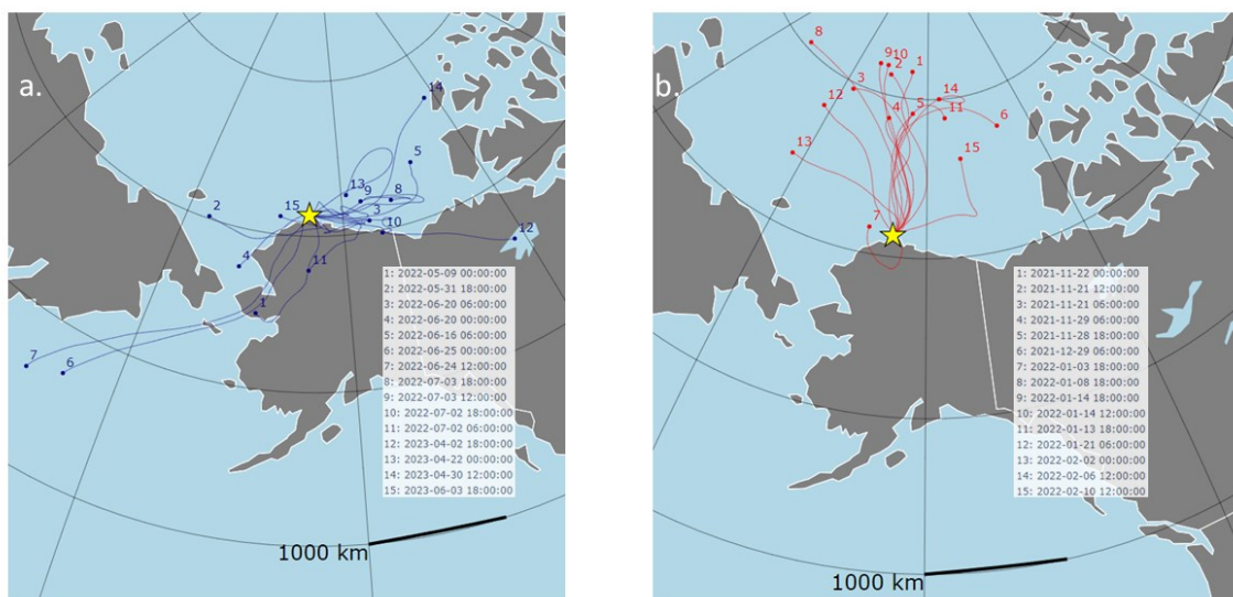
195 Figure S6. Air mass origins and back trajectories at the inlet height from BRW (yellow star). The air mass trajectories during high- and low-INP episodes are shown in blue and red colors. Panel (a) represents the data selected with a low – high threshold of the 25 th – 75 th percentile based on n_s , at all -30 , -25 , and -20 °C (below or above at ‘all’ temps). Panel (b) represents the data selected with a low – high INP threshold of the 25 th – 75 th percentile based on n_s(T) at all selected temperatures.
