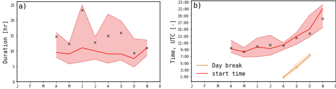
Fig 3: (a) the duration of the entire growth of newly formed particles from the first measurable size bin i.e. 2.5nm to the largest size bin (b) the average start time of the observed new particle formation (NPF) (monthly mean displayed by the cross and median by the red line), along with a shaded region representing the 25 th and 75 th percentiles. Along with the estimated time the global horizontal irradiance (GHI) goes beyond zero (i.e. daybreak). The average time of day break for the months April until July is not applicable, since the sun is constantly above the horizon (as experienced by ZEP). Time is given in terms of coordinated universal time (UTC).
