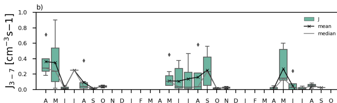
Fig 4: a) the calculated growth rates (GRs) b) calculated median formation rates for particles between 3 and 7nm ( J_{\text{med}, 3-7} ) throughout the measurement period are represented by box-whiskers, which display the monthly growth rate averages and include the median and 25 th - 75 th percentiles. The green box-whiskers refer to the average GRs/ J_{3-7} s from the start of the NPF until it stops growing. The black line cross represents the mean, and the grey lines join the median values. Diamonds represent outliers.
