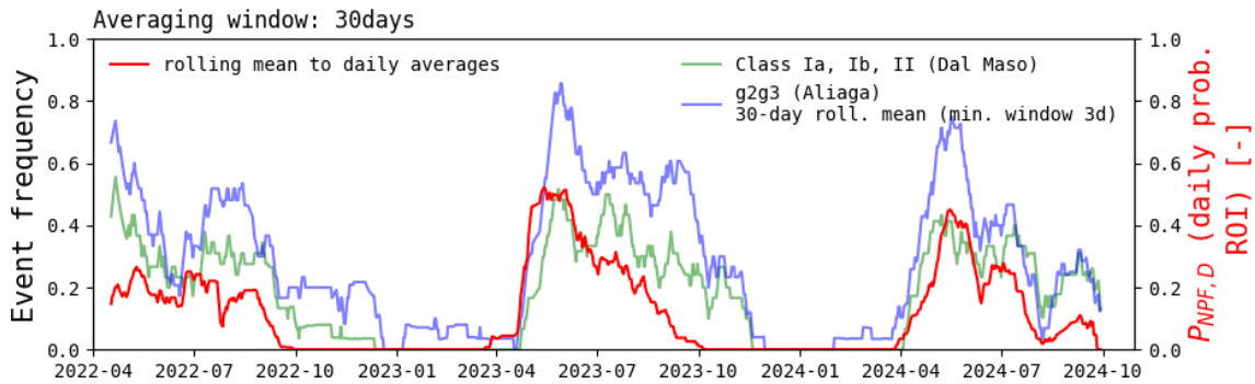
Fig 10: The red line is P_{NPF,D} , the estimated daily likelihood of measurements occurring in the region of interest (ROI). The ROI is based on the relation between CS and 6-hour solar accumulation and is defined in Fig. 8). The green and blue lines represent the rolling averages of the NPF daily event frequencies using the Dal Maso et al. (2005) and Aliaga et al. (2023) classification respectively. The green and blue curves are present here to be able to compare to P_{NPF,D} (daily prob. ROI).
