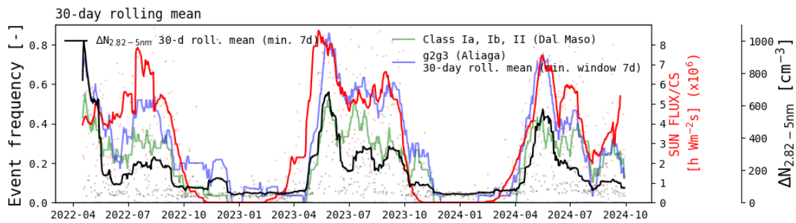
Fig 11: The red line is the solar insolation divided by the condensation sink (Solar insolation/CS) with a 30-day rolling mean. The intensity parameter ( \Delta N_{2.82-5nm} ). The green and blue lines represent the rolling averages of the NPF daily event frequencies using the Dal Maso et al. (2005) and Aliaga et al. (2023) classification respectively. The green and blue curves are present to be able to compare to the red line representing a proxy for the balance between sources and sinks.
