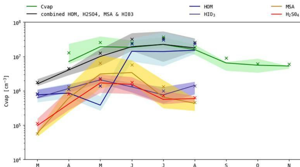
Fig 5: Estimated concentration of condensable vapours ( C_v , green) compared with measured concentrations: the monthly means (crosses) and medians (thick line), along with the 25 th and 75 th percentiles (shaded region) for both
