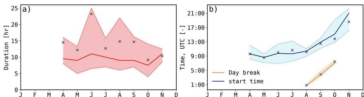
Fig 3: (a) duration of the entire growth of newly formed particles from the first measurable size bin i.e. 2.5nm to the largest size bin (b) average start time of the observed new particle formation event (NPF). Monthly means displayed by crosses and medians by the red and blue lines respectively, along with a shaded region representing the 25 th and 75 th percentiles. Time when the global horizontal irradiance (GHI) is greater than zero (i.e. Day break) is displayed in orange. The average Day break time for the months April until July is not applicable, since the sun is constantly above the horizon (as experienced by ZEP during the polar day). Time is given in terms of coordinated universal time (UTC).
