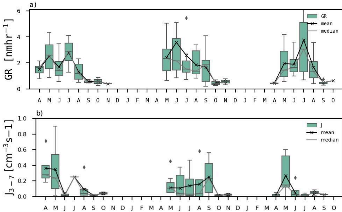
Fig 4: a) the calculated growth rates (GRs) b) calculated median formation rates for particles between 3 and 7nm ( J_{\text{med}, 3-7} ) throughout the measurement period are represented by box-whiskers, which display the monthly growth rate averages and include the median and 25 th - 75 th percentiles. The green box-whiskers refer to the average GRs/ J_{3-7} s from the start of the NPF until it stops growing. The black line cross represents the mean, and the grey lines join the median values. Diamonds represent outliers.
