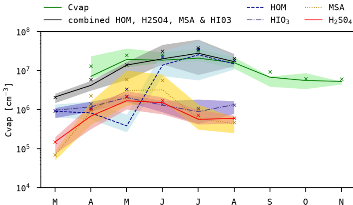
Fig 5: Estimated concentration of condensable vapours (Cv, solid green) compared with measured concentrations: the monthly means (crosses) and medians (thick line), along with the 25 th and 75 th percentiles (shaded region) for both Cv and Ny-Ålesund measurements. Arctic precursor vapours namely sulphuric acid ( \text{H}_2\text{SO}_4 , solid red), methanesulphonic acid (MSA, dotted gold), highly oxygenated molecules (HOM, dashed dark blue) and iodic acid ( \text{HIO}_3 , dash dot purple) and combined (grey) from Beck et al. (2021) are displayed. The estimated Cv measurements cover the years 2022 to 2024, whilst the Svalbard measurements from Beck et al. (2021) cover the period 2017-03-22 to 2017-08-23.
