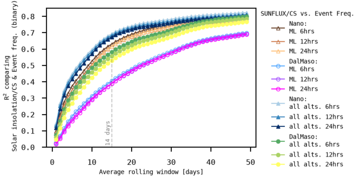
Fig. 12: Correlation between the event frequency (either defined using the Dal Maso, circles or Nano ranking, triangles, classification method) and the ratio of the accumulated solar insolation and CS (SUNFLUX/CS) with a rolling average applied. The coefficient of determination ( R^2 ) is a function of the rolling window size (i.e., number of days). The first 6, 12, and 24 hours of the back trajectories are selected (in different shades). The curve labelled ML (empty symbols) represents back trajectories that traversed only through the mixed layer, while the curves labelled all alts. (whole symbols) represent back trajectories at all altitudes. Grey dashed line at 14 days to indicate plateauing of R^2 .
