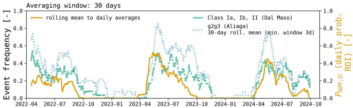
Fig 10: The orange line is P_{NPF,D} , the estimated daily likelihood of measurements occurring in the region of interest (ROI). The ROI is based on the relation between CS and 6-hour solar accumulation and is defined in Fig. 8). The green dash-dot and blue dotted lines represent the rolling averages of the NPF daily event frequencies using the Dal Maso et al. (2005) and Aliaga et al. (2023) classification respectively. The green and blue curves are present here to be able to compare to P_{NPF,D} .
