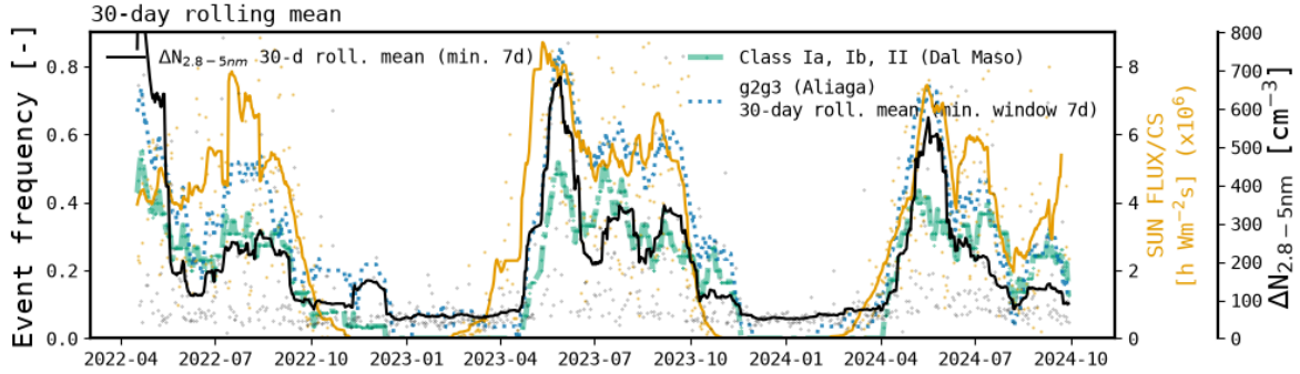
Fig 11: The solar insolation divided by the condensation sink (Solar insolation/CS, SUN FLUX/CS) with a 30-day rolling mean, is denoted by the orange line. The intensity parameter ( \Delta N_{2.8-5nm} ) is shown in black. The green dash-dot and blue dotted lines represent the rolling averages of the NPF daily event frequencies using the Dal Maso et al. (2005) and Aliaga et al. (2023) classification schemes respectively. The green and blue curves are displayed to be able to compare to the orange line, the proxy for NPF activity i.e. the balance between sources and sinks.
