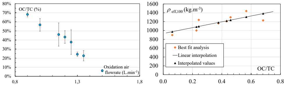
550 Figure 7 – Evolution of the OC/TC ratio as a function of the oxidation air flowrate (left). Identification of \rho_{eff,100} as a function of OC/TC ratio.
