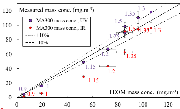
Figure 2 – Mass concentrations measured by the MA300 as a function of the TEOM reference measurements.
