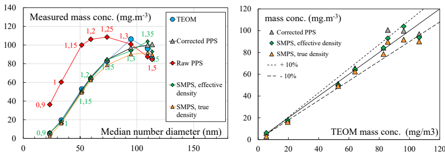
555 Figure 8 – Comparison of gravimetric mass concentrations with evaluations based on PPS and SMPS measurements.
