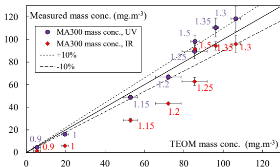
520 Figure 9 – Mass concentrations measured by the MA300 as a function of the TEOM reference measurements
