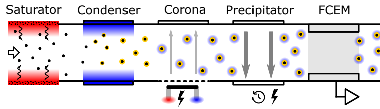
Figure 1. Schematic drawing of the CDC. The carrier gas is saturated after entering the device and then cooled in the condenser to induce supersaturation and subsequent particle growth. The enlarged particles then enter the detector section, where they are charged by ions from an external high-voltage corona which are drawn into the flow path with a small voltage. The charged particles are then periodically precipitated and finally counted by a Faraday cup electrometer (FCEM).
