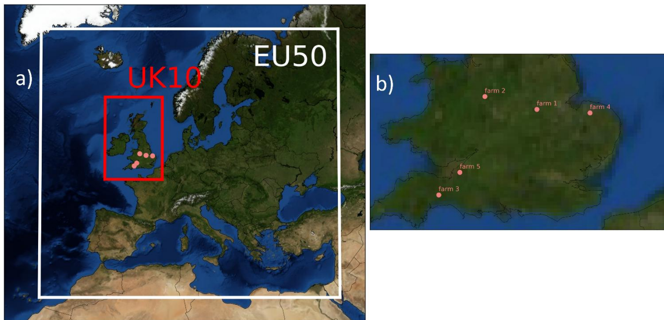
190 Figure 1: a) Regional nested modelling domains and location of the studied farms. The white box corresponds to the European domain at 50 km × 50 km horizontal resolution (EU50) and the red box to the UK domain at 10 km × 10 km horizontal resolution (UK10). Each farm is shown with a pink coral circle. b) Zoom on the location of each studied farm with their corresponding id. The details on the farms are provided in Table 2.
