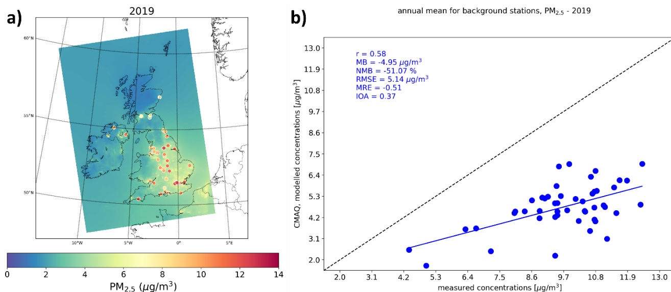
385 Figure 3: a) Spatial distribution of annual mean \text{PM}_{2.5} concentrations in \mu\text{g}/\text{m}^3 calculated by CMAQ at 10 km resolution in 2019. The measured concentrations at the monitoring stations are shown with the coloured circles. b) Comparison between these annual measured concentrations with the modelled values in 2019. Only the background stations with a data capture higher than 75% are used. Insert values are the Pearson correlation coefficient (R), the mean bias (MB), the normalized mean bias (NMB), the mean relative error (MRE), the root-mean-square error (RMSE), and the index of agreement (IOA). The blue line represents the linear fit and dashed black line is the 1:1 slope.
