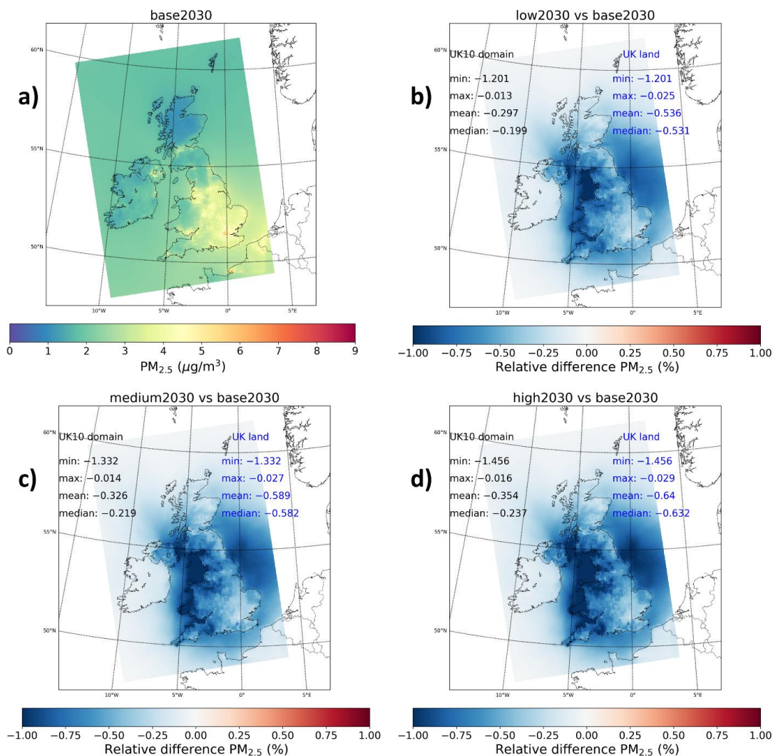
Figure 4: a) Spatial distribution of annual mean PM 2.5 concentrations in µg/m 3 calculated by CMAQ at 10 km resolution for the base2030 scenario. Relative difference of the same distribution with the low2030 (b), medium2030 (c) and high2030 (d) scenarios. The minimum, maximum, mean, and median relative difference values in the whole UK10 domain (in black) and for the UK land grid cells (blue) are provided. The relative difference is calculated as follow: ((scenario-base)/base) × 100%.
