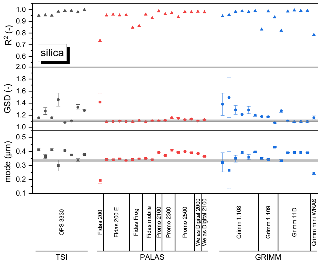
190 Figure 4. PNSD parameters (mode, GSD) and lognormal model fit quality ( R^2 ) for monodisperse silica for the different instruments involved in the ILC. The grey area corresponds to the 90% confidence interval of the parameters obtained with the control instrument.
