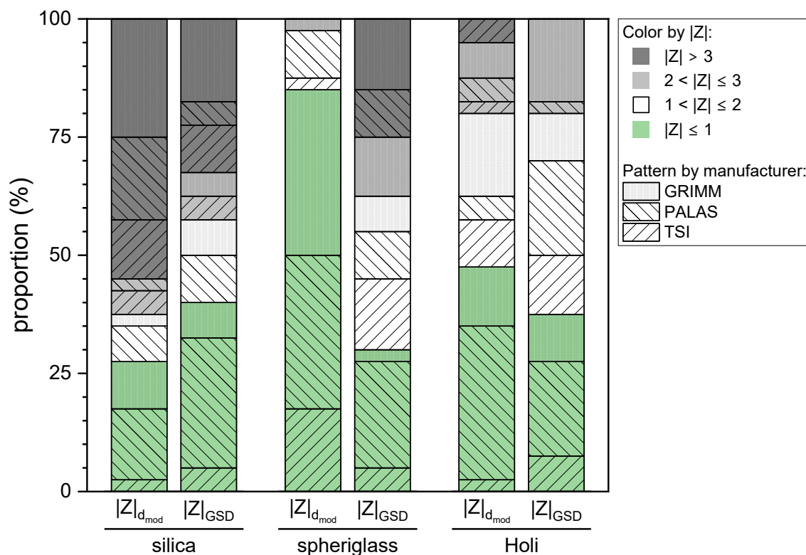
Figure 7. Z-score calculated for each OPSS tested in the interlaboratory comparison for the three test aerosols (silica, spheriglass, Holi powder) in function of each manufacturer (TSI, PALAS, GRIMM).
