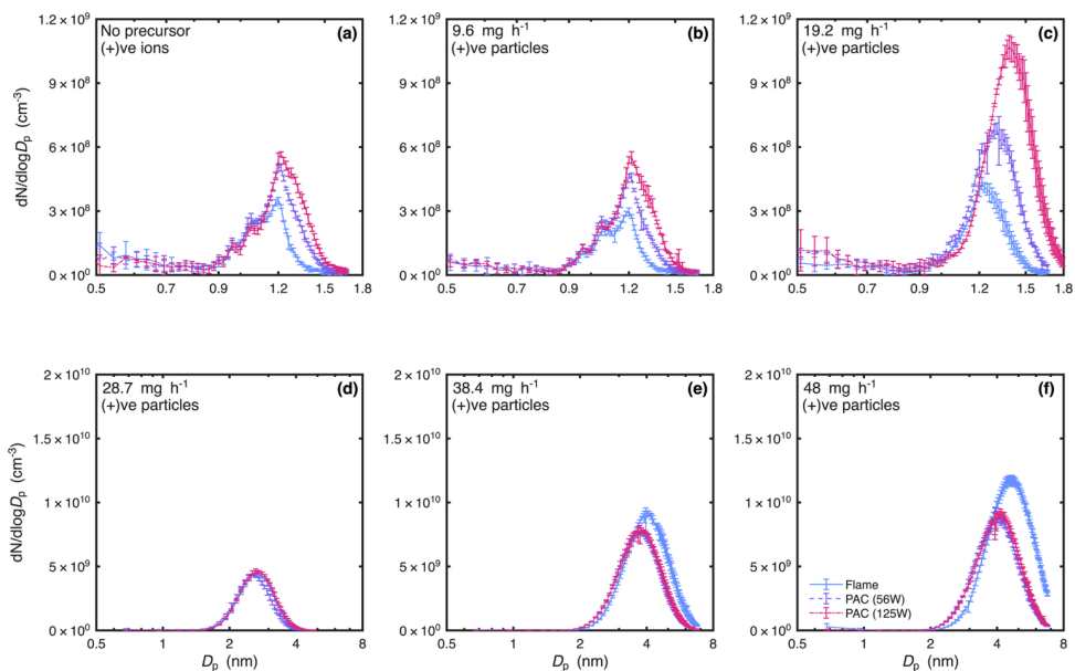
415 Figure 3: (a) The size distribution of positive ions without any TTIP; (b), (c), (d), (e), and (f) are the size distribution of positively charged Ti-containing clusters with TTIP feed rates ranging from of 9.6 mg h -1 to 48 mg h -1 . Each panel compares the influence of corona discharge at power 56 W and 125 W on the size distribution. Error bars denote the standard deviation.
