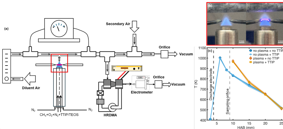
Figure 1: (a) Schematic of the experimental apparatus, with a red box highlighting the flame and corona discharge region, (b) Image of flame with and without a corona discharge in the highlighted region. (c) Temperature profile of flames under different plasma and synthesis precursor conditions. The feed rate of TTIP is 19 \text{ mg h}^{-1} for temperature profile measure, and the plasma power is 125 W.
