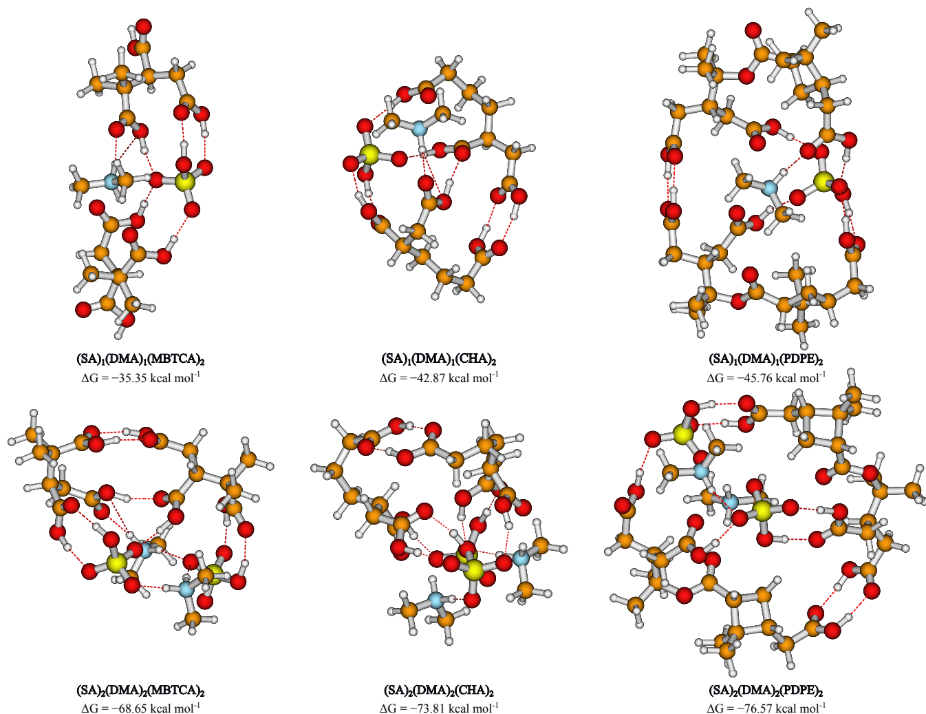
Figure 6. The (SA) 1 (DMA) 1 (OOM) 2 and (SA) 2 (DMA) 2 (OOM) 2 cluster geometries lowest in binding Gibbs free energy at the DLPNO-CCSD(T 0 )/aug-cc-pVTZ// \omega B97X-D/6-31++G(d,p) level of theory with a quasi-harmonic threshold of 100 cm -1 , at 298.15 K and 1 atm. Orange is carbon, red is oxygen, blue is nitrogen, yellow is sulfur, and white is hydrogen.
