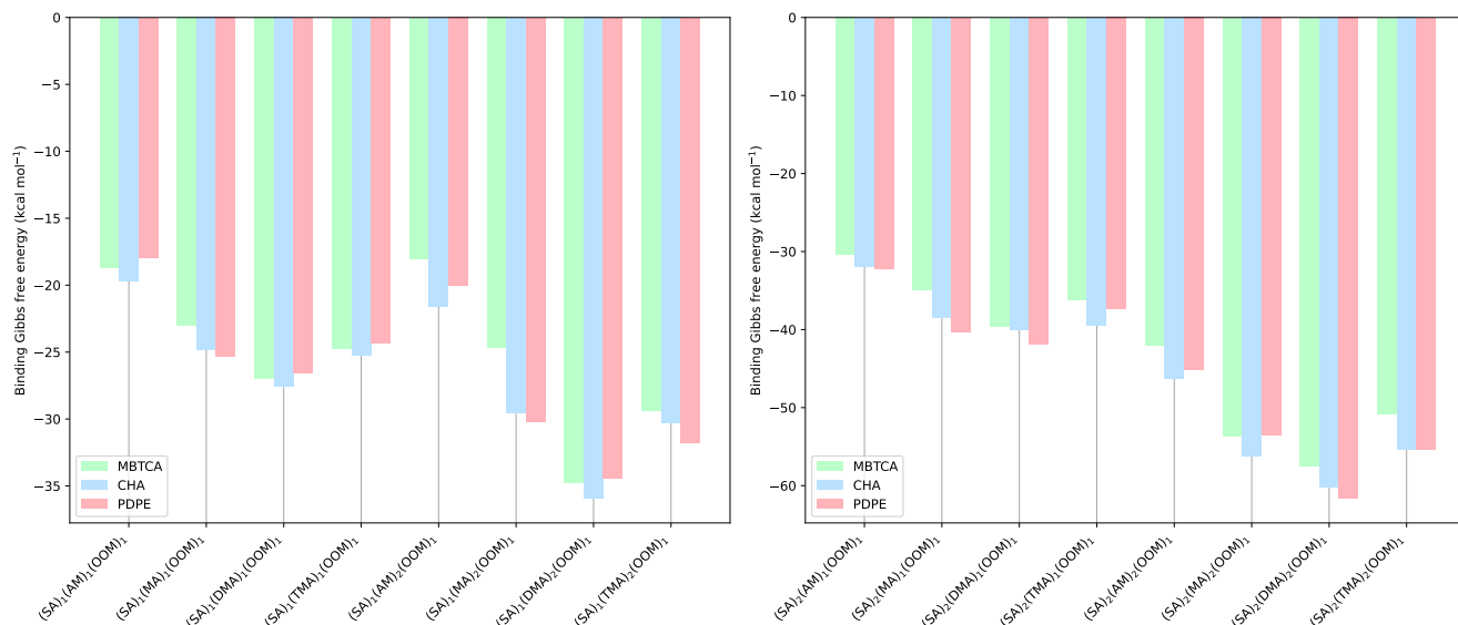
Figure 3. The binding Gibbs free energy of the (SA)_{1-2}(Base)_{1-2}(MBTCA)_1 , (SA)_{1-2}(Base)_{1-2}(CHA)_1 and (SA)_{1-2}(Base)_{1-2}(PDPE)_1 clusters, calculated at the DLPNO-CCSD( T_0 )/aug-cc-pVTZ// \omega B97X-D/6-31++G(d,p) level of theory with a quasi-harmonic threshold of 100\text{ cm}^{-1} , at 298.15 K and 1 atm. The left panel shows clusters with 1 SA, the right panel shows clusters with 2 SAs.
