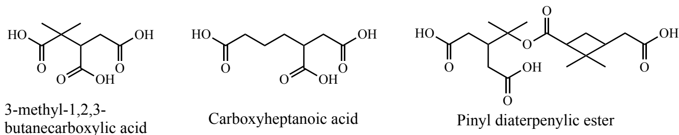
Figure 1. Molecular structure of the three organic molecules studied MBTCA, CHA and PDPE.
