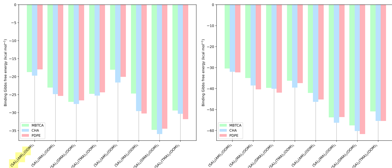
Figure 3. The binding Gibbs free energy of the (\text{SA})_{1-2}(\text{Base})_{1-2}(\text{MBTCA})_1 , (\text{SA})_{1-2}(\text{Base})_{1-2}(\text{CHA})_1 and (\text{SA})_{1-2}(\text{Base})_{1-2}(\text{PDPE})_1 clusters, calculated at the DLPNO-CCSD( T_0 )/aug-cc-pVTZ// \omega B97X-D/6-31++G(d,p) level of theory with a quasi-harmonic threshold of 100 \text{ cm}^{-1} , at 298.15 K and 1 atm.
