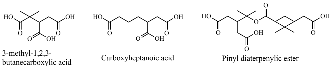
Figure 1. Molecular structure of MBTCA, CHA and PDPE.
