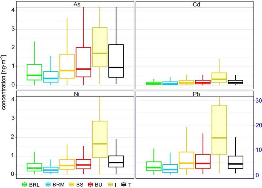
Figure 3: HM concentration overview at all station types, 2010–2021. Colours represent particular station types. Background Rural Lowland stations (BRL) in green, Background Rural Mountain stations (BRM) in light blue, Background Suburban stations (BS) in orange, Background Urban stations (BU) in red, Industrial station (I) in yellow, and Traffic station (T) in black.
