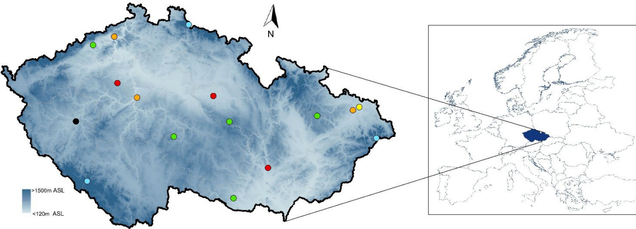
125 Figure 2: Spatial distribution of selected stations measuring HM in the period of 2010–2021 in the Czech Republic, Europe. Colours represent particular station types. Background Rural Mountain stations (BRM) are coloured light blue, Background Rural Lowland stations (BRL) in green, Background Urban stations (BU) in red, Background Suburban stations (BS) in orange, Industrial station (I) in yellow and Traffic station (T) in black. ASL denotes metres above sea level . The map data were processed in ArcGis-ArcGIS software, © Esri, 2018. All rights reserved. ; ASL denotes metres above sea level (ESRI, 2018).
