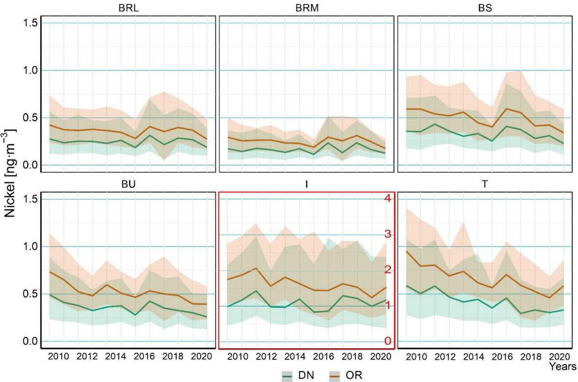
305 Figure 7: Nickel concentration at Background Rural Lowland stations (BRL), Background Rural Mountain stations (BRM), Background Suburban stations (BS), Background Urban stations (BU), Industrial station (I) and Traffic station (T), 2010–2021. The green line represents the median concentration of dispersion normalising data (DN), and the orange line, the median concentration of the original data series (OR). The coloured area visualises the interquartile range (25 th –75 percentile).
