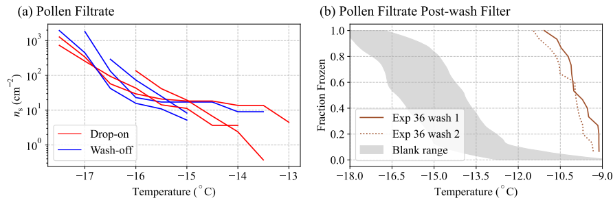
Figure 6. INP experiments and washed filter punch results for pollen filtrate. The wash-off and drop-on techniques report similar activity, despite INPs remaining on the washed filter punches. (a) Active Site Density versus Temperature for the pollen filtrate experiments and (b) the IR-NIPI results for the washed polycarbonate filter punches from experiment 36.
