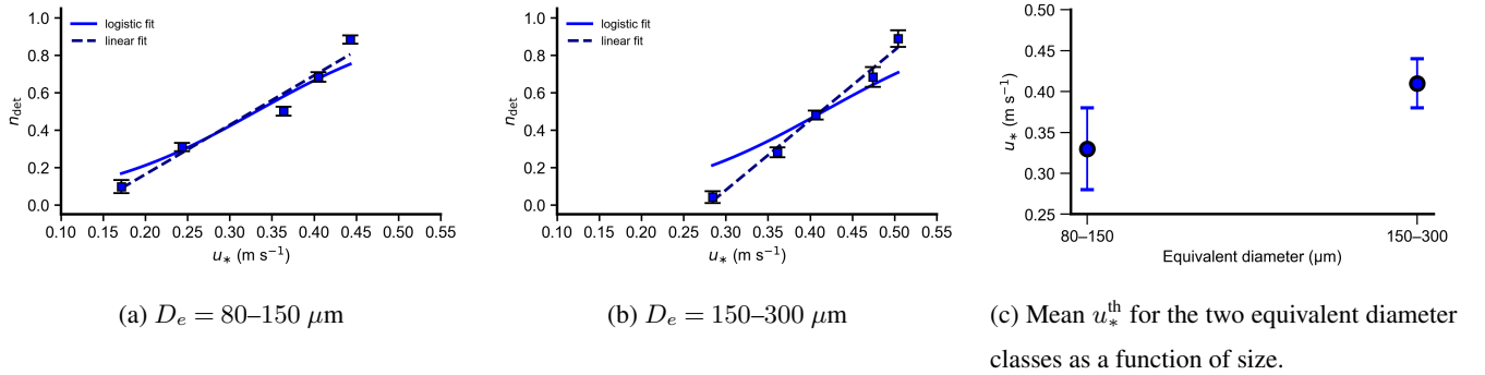
Figure 13. Size-resolved detachment behaviour of TWPs on the glass substrate. Panels (a) and (b) show the normalized detachment fraction ( n_{\text{det}} ) as a function of friction velocity for the two equivalent diameter class ( D_e = 80\text{--}150\ \mu\text{m} and 150\text{--}300\ \mu\text{m} ). Squares denote ensemble means and error bars denote \pm 1 SD of the binned data; solid and dashed lines indicate the logistic and linear regression fits, respectively. Panel (c) compares the mean threshold friction velocity for the two size classes; error bars denote \pm 1 SD across samples.
