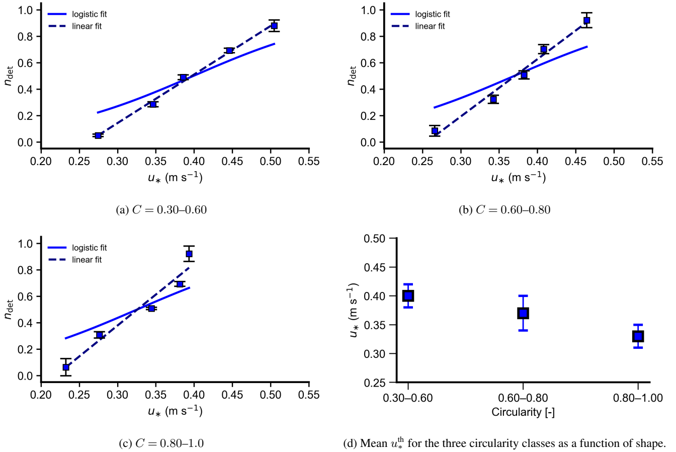
Figure 14. Shape-resolved detachment behaviour of TWPs on glass substrate. Panels (a)-(c) show the normalized detached fraction as a function of friction velocity for the three circularity classes ( C = 0.30-0.60 , 0.60-0.80 , 0.80-1.00 ). Squares denote ensemble means \pm 1 SD of the binned data; solid and dashed lines indicate the logistic and linear regression fits, respectively. Panel (d) shows the mean threshold friction velocity of the three shape classes; error bars denote \pm 1 SD across samples.
