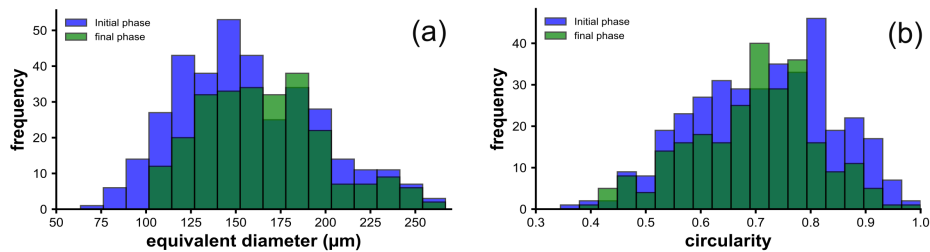
Figure D3. Comparison of particle morphology distribution at initial and final phase of detachment. (a) projected equivalent diameter (b) circularity. Blue histograms represent the initial deposited population (initial phase), while the green histograms represent the particles remaining at the end of the detachment experiment (final phase). The shift in the final distributions relative to the initial population, indicating selective detachment with respect to morphology. Larger particle size remained attached, whereas more rounded (higher circularity) particles were preferentially detached.
