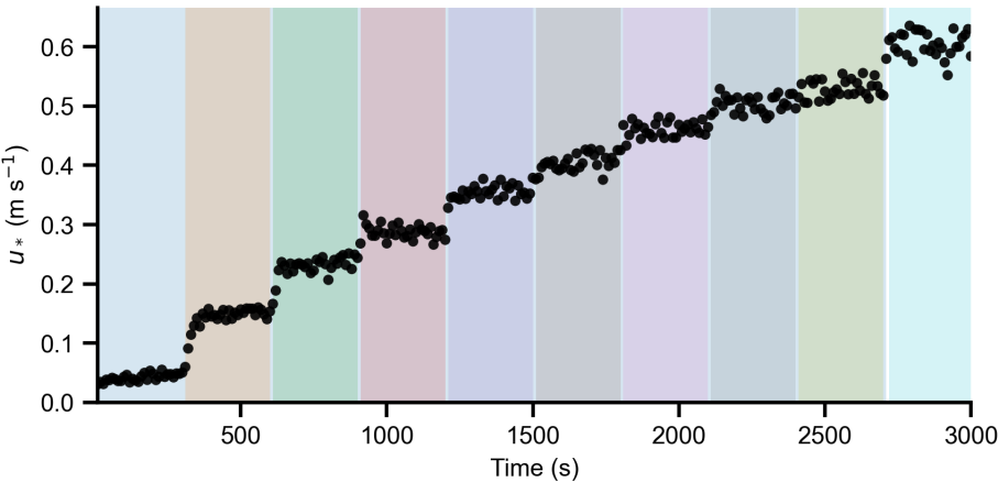
Figure D1. Friction-velocity time series used in the detachment protocol at z = 1.4 cm. Black markers show the instantaneous u_*(t) , while the shaded background bands denote the successive flow stages. Each stage corresponded to an exposure time of 300 s, followed by a discrete change to the next stage. Stage changes were characterized by a short transient adjustment of u_* before reaching a quasi-steady level within each stage.
