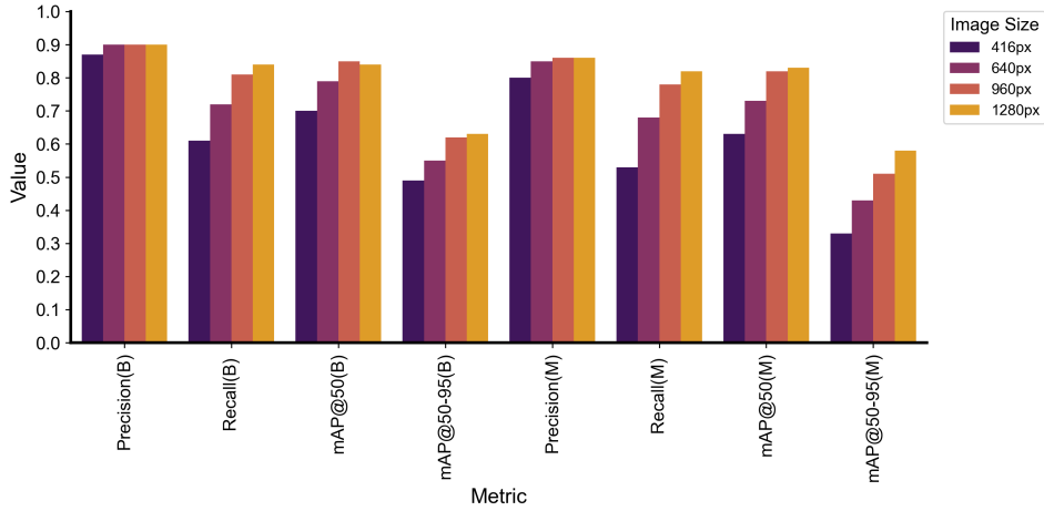
Figure 5. Comparison of model performance across input image resolutions. The figure evaluates the performance for TWP detection and segmentation at four input image sizes (416 px, 640 px, 960 px, and 1280 px). Metrics labelled B refer to bounding-box predictions and M as mask predictions. Results illustrates how image resolution impacts detection and segmentation accuracy.
