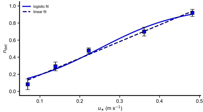
Figure 12. Detached fraction of TWPs, normalized to the maximum in each replicate, as a function of friction velocity ( u_* ) for the eight replicates. The data points show ensembled averaged values (mean \pm SD across samples). The solid line is the logistic fit ( R^2 = 0.97 ); the dashed line is linear regression fit ( R^2 = 0.98 ).
