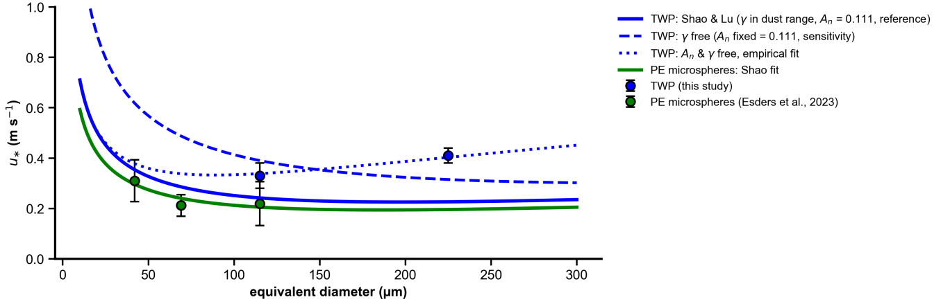
Figure 15. shows the threshold friction velocity u_*^{\text{th}} as a function of projected equivalent diameter D_e for TWPs (blue circles), and PE polyethylene microspheres (green circles; data from Esders et al. (2023)) on glass substrate. Error bars denote \pm 1 SD). The solid blue line shows the Shao Lu model fit with dust parameter range, the dashed blue line shows a fit with A_N fixed and (\gamma) adjusted, and the dotted blue line shows the fit with both A_N and (\gamma) adjusted. The solid green line is the Shao and Lu fit for the PE polyethylene microsphere data.
