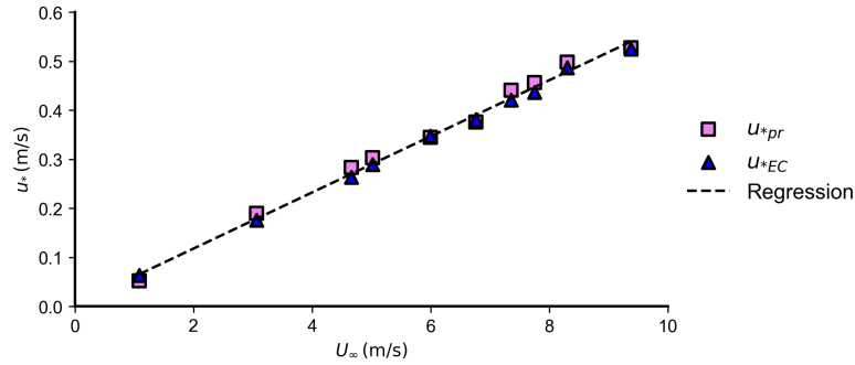
Figure 9. Calibration of u_* from the profile measurement and eddy-covariance as a function of free-stream velocity at z = 0.0114 m. The regression gives R^2 = 0.994 , with a 95% confidence interval of 0.055–0.059 for the fitted coefficient.
