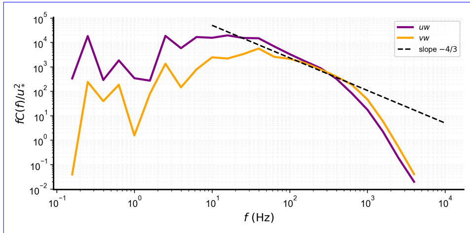
Figure C4. co-spectra normalized by the the square of the friction velocity , plotted as fC(f)/u_*^2 against frequency f . The co-spectra ( uw , vw ) are shown at the measurement height of z = 1.4\text{cm} for the highest windspeed stage. The dashed line indicates a reference slope of -4/3 , corresponding to the expected inertial subrange .
