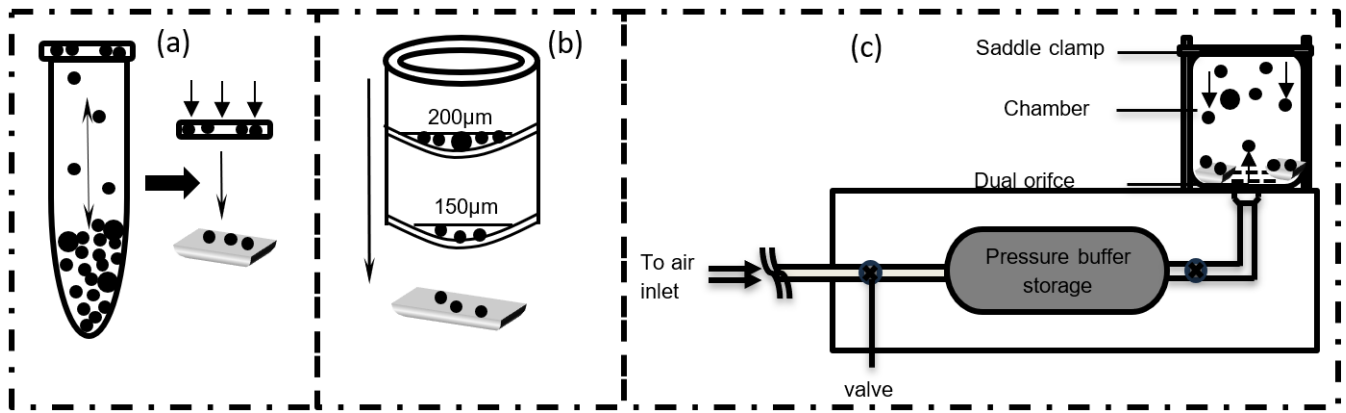
Figure 4. Diagram illustrating the three seeding methods. (a) cap tipping method (b) sieving method (c) developed low cost pressurized method
