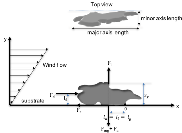
Figure 10. Simplified two-dimensional conceptual schematic of the principal forces acting on nonspherical non-spherical particles on a surface, includes the aerodynamic; drag force ( F_d ), lift ( F_l ), stabilizing; adhesion force ( F_a ), gravitational force ( F_{mg} ), and frictional force ( F_r ), adapted from Olivares et al. (2024). This figure illustrates the force-balance framework considered in this study. When the moment of the aerodynamic forces exceeds the stabilizing forces, the particle detaches and gets entrained into the flow.
