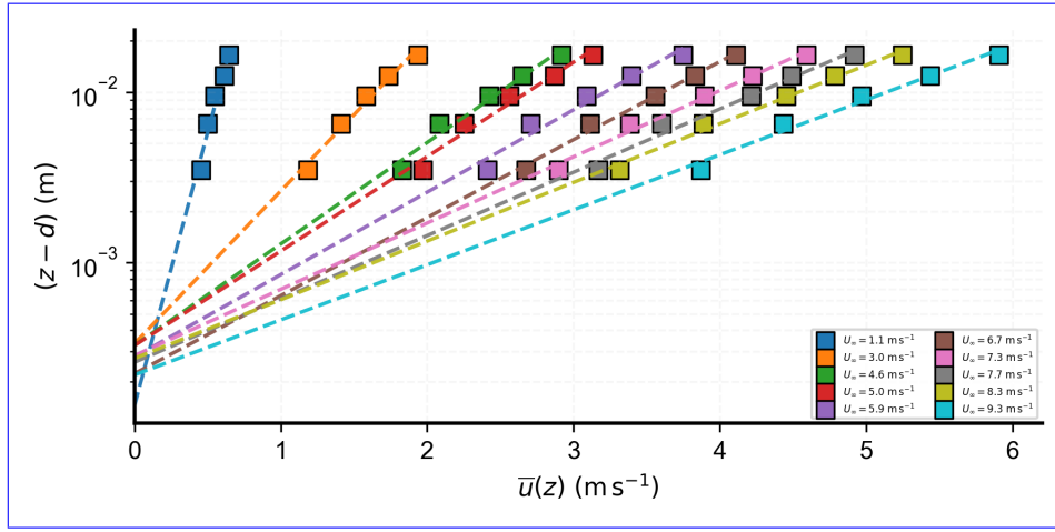
Figure 8. Logarithmic wind profile plots showing the relationship between the mean wind speed \bar{u}(z) and logarithmic height \ln(z-d) across the ten flow stages. Each colour represents one stage, and the dashed lines indicate the logarithmic fits used to derive the profile based friction velocity ( u_* ) with ( \kappa = 0.4 ). Extrapolating the data to U = 0 yields the roughness lengths ( z_0 \approx 0.3 mm).
