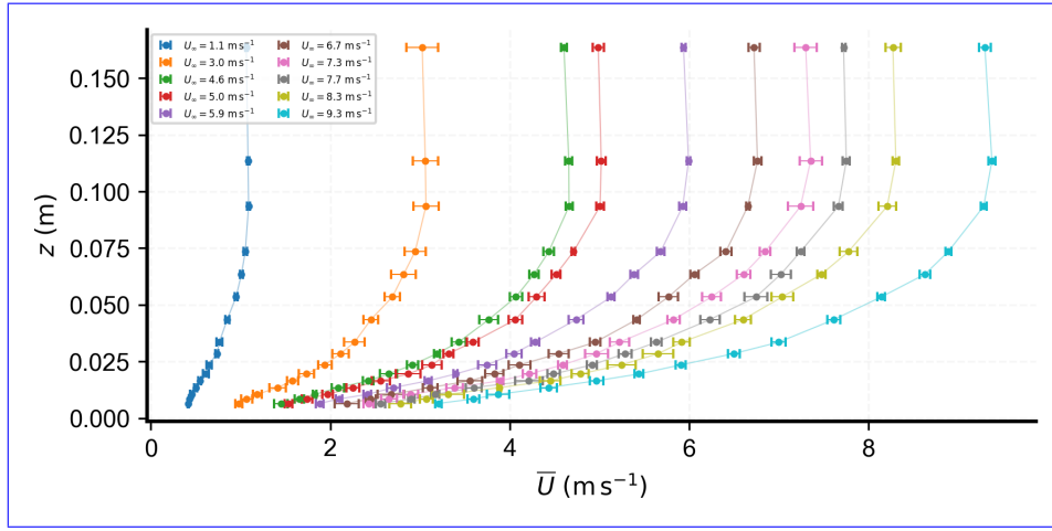
Figure C1. Vertical wind profile of the mean streamwise velocity \bar{U} , measured across the ten stepwise flow stages. Symbols represent the mean values at each measurement height, with the error bars indicating the standard deviation across the four replicates. These profiles show the progressive increase in the flow speed with stage.
