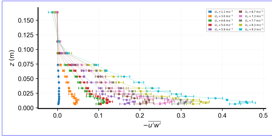
Figure C2. Vertical shear stress profile -\overline{u'w'} , measured across the ten flow stages, with symbols representing the mean values and error bars also indicating the standard deviation across four replicates. The magnitude of the shear stress generally increases towards the wall within the roughness-influenced layer, indicating enhanced downward momentum transfer near the surface.
