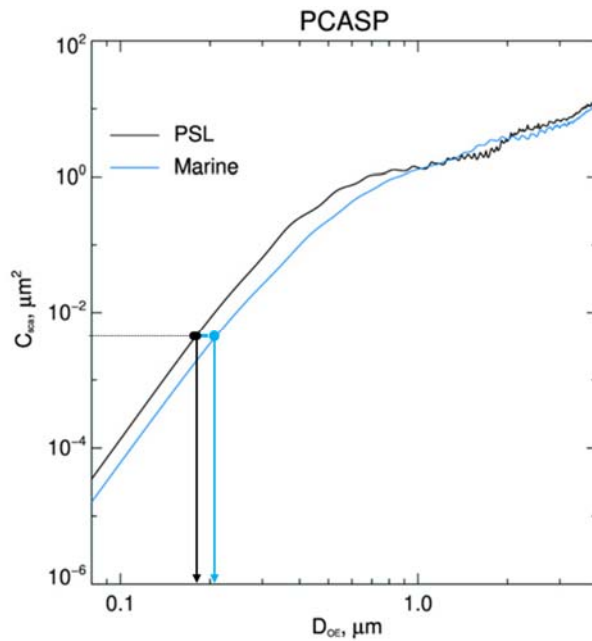
244 Figure 1. Scattering cross section C_{sca} as a function of particle diameter calculated using Mie theory for the PCASP. 245 The black line represents the C_{sca} for the calibration particles (PSL). The light blue line represents the C_{sca} for 246 marine aerosols ( m = 1.38 - 0.001i ). The small vertical grey lines represent the bin edges for the nominal calibration 247 particles.
