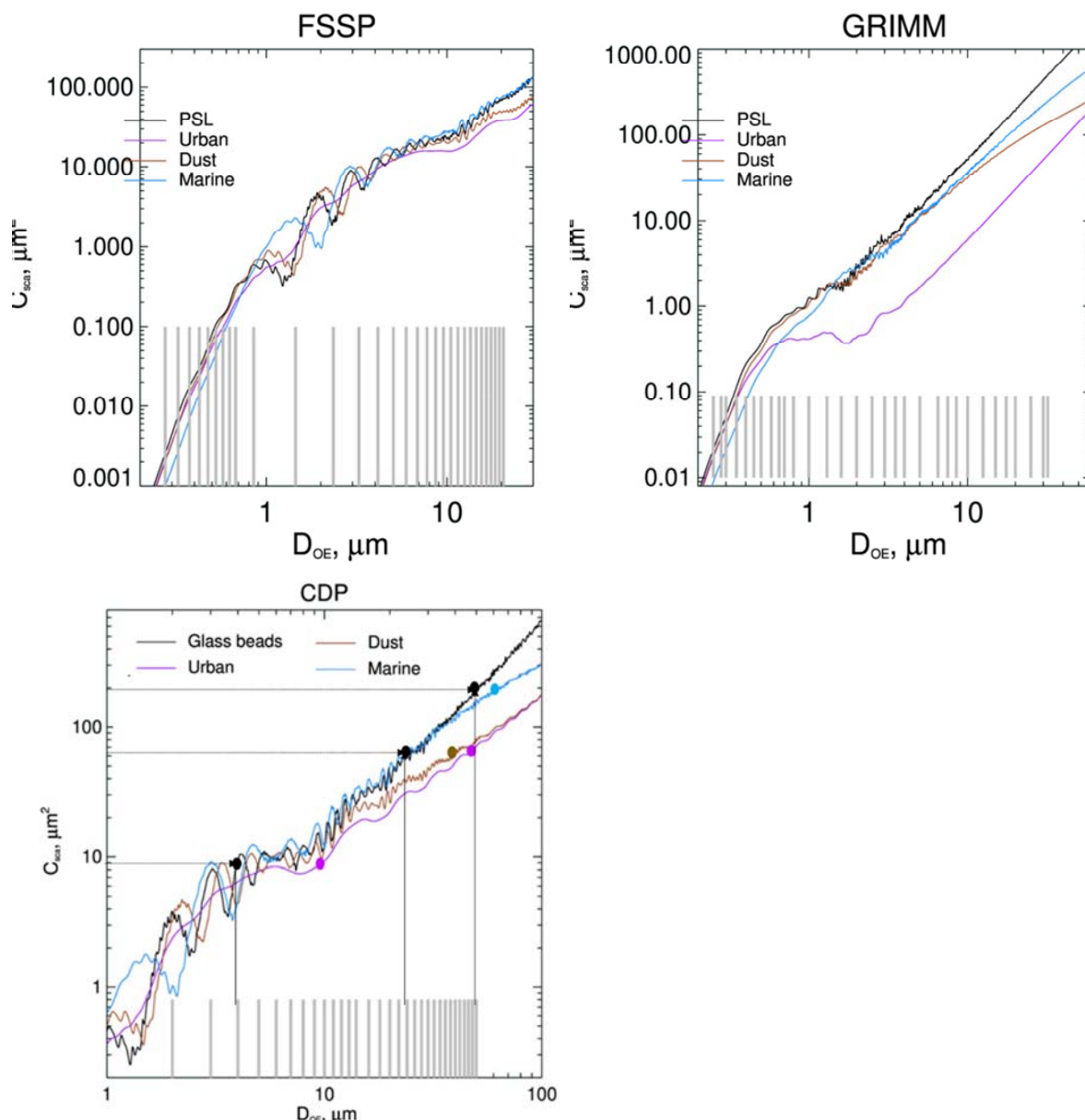
Figure 2. Scattering cross section C_{sca} as a function of particle diameter calculated using Mie theory for the OPCs considered in this paper. The black lines represent C_{sca} for the calibration particles (PSL or glass beads). The purple lines represent the C_{sca} function for absorbing urban aerosols ( m = 1.56 - 0.087i ), while the brown lines represent C_{sca} for moderately-absorbing mineral dust ( m = 1.53 - 0.003i ), and the light blue lines represent C_{sca} for marine aerosols ( m = 1.38 - 0.001i ). The small vertical grey lines represent the bin edges for each OPC.
