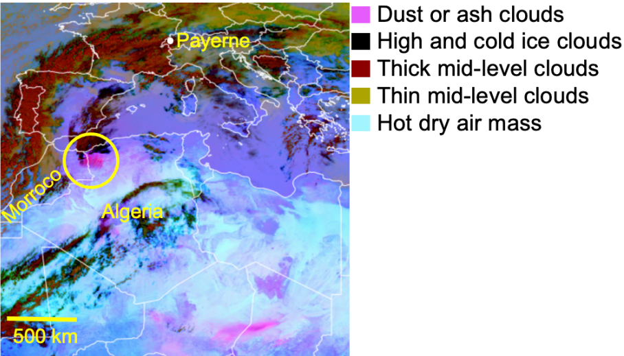
Figure 3: Satellite RGB image (5.2.2021, 22:00 UTC) from the SEVIRI dust product. The dust plume transported to central Europe is seen east of the Moroccan – Algerian border (center of yellow circle).
