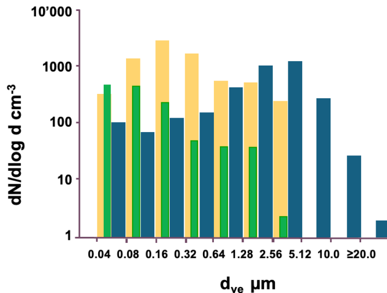
Figure 10: Jungfrauoch PSD measured in April 2004, when JFJ was above the PBL, cloud-free, and no SDE (green bars); during the SDE of February 6th at 12:00 (yellow bars, shifted 1 bin to the left relative to the original data, see text); and for an iberulite sample collected in St. L  gier (blue bars).
