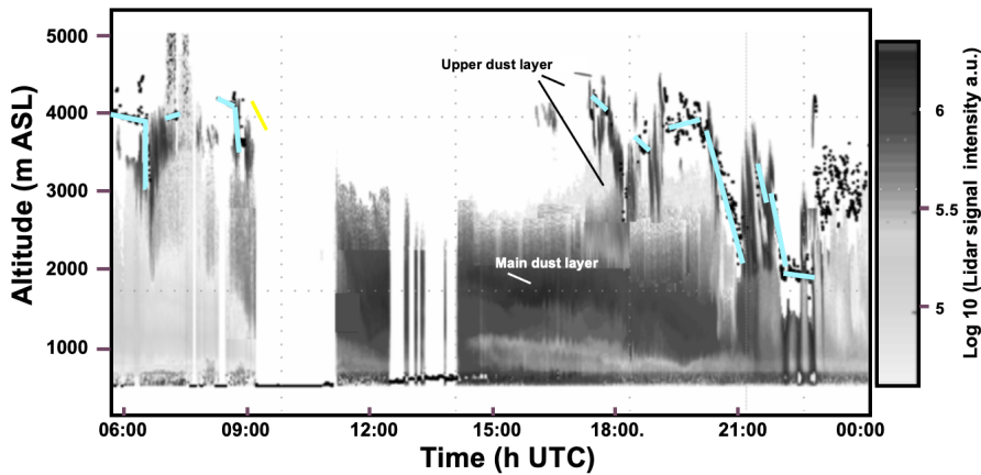
Figure 5: Ceilometer profile for February 6th (MeteoSwiss). The small black dots and blue lines above the reflections indicate the meteorological cloud base. The white strips are gaps due to ground fog.
