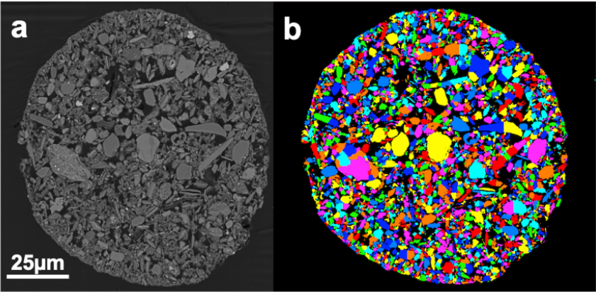
Figure 8: SEM images of some iberulites collected in St L  gier on February 6th, 2021. Figure (f) shows the fine-grained rim and the coarse core of an iberulite.
