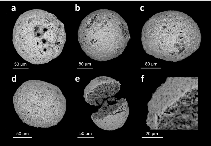
Figure 8: SEM images of some iberulites collected in St L  gier on February 6th, 2021. Figure (f) shows the fine-grained rim and the coarse core of an iberulite.
