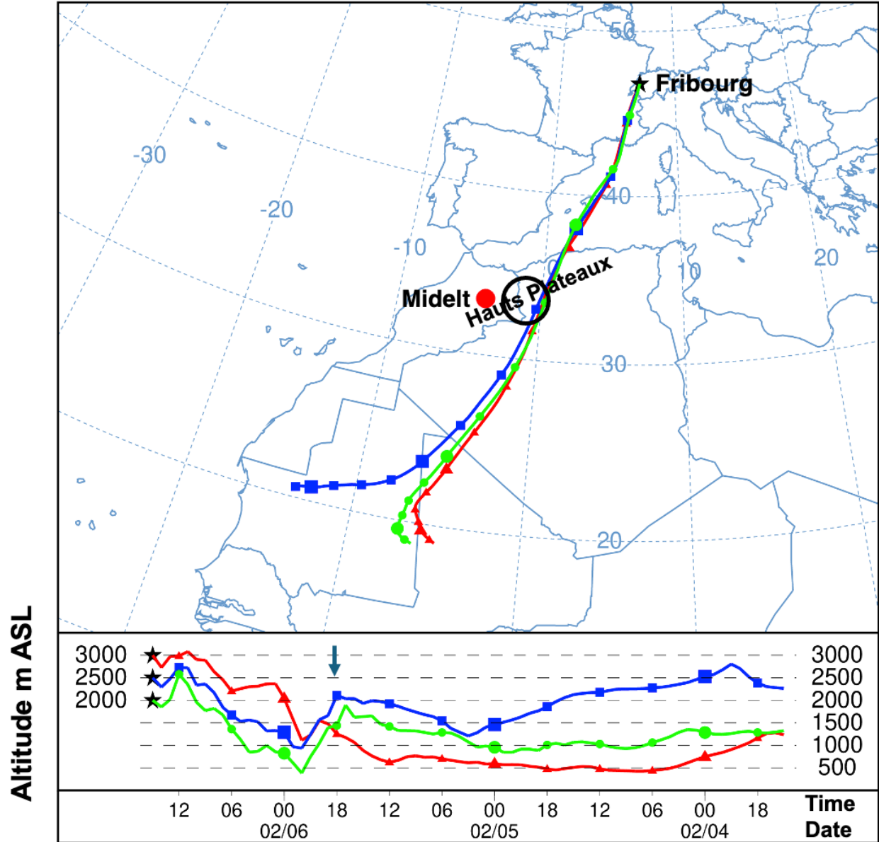
Figure 2: Back trajectories for air masses arriving over Payerne at 15:00 UTC, February 6 th . The black circle shows the location of the first appearance of the dust plume entrained across the Mediterranean Sea towards central Europe. Midelt is the location where meteorological during the pick up of the dust are known. The black arrow points to the location markers inside the black circle e.g. close to the dust plume visible in Figure 2 (yellow circle).
