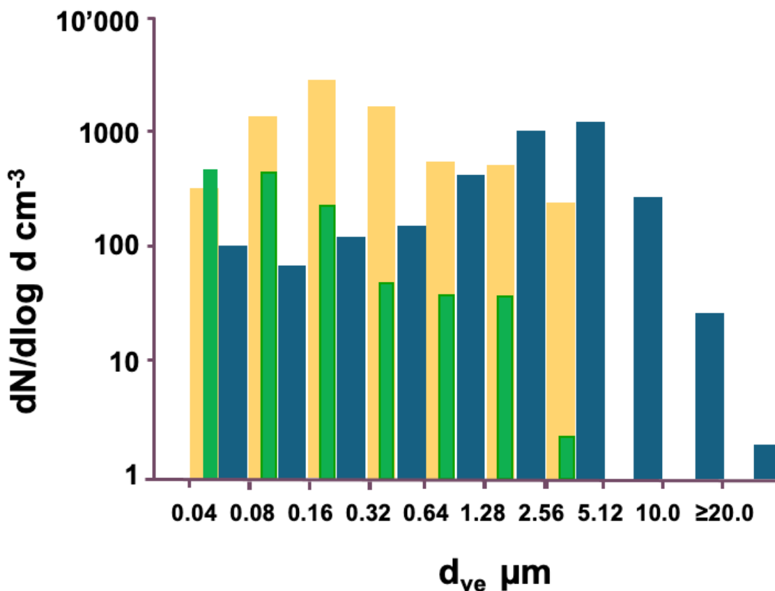
Figure 10: Jungfraujoeh PSD measured in April 2004, when JFJ was above the PBL, cloud-free, and no SDE (green bars); during the SDE of February 6th at 12:00 (yellow bars, shifted 1 bin to the left relative to the original data, see text); and for an iberulite sample collected in St. Léger (blue bars).
