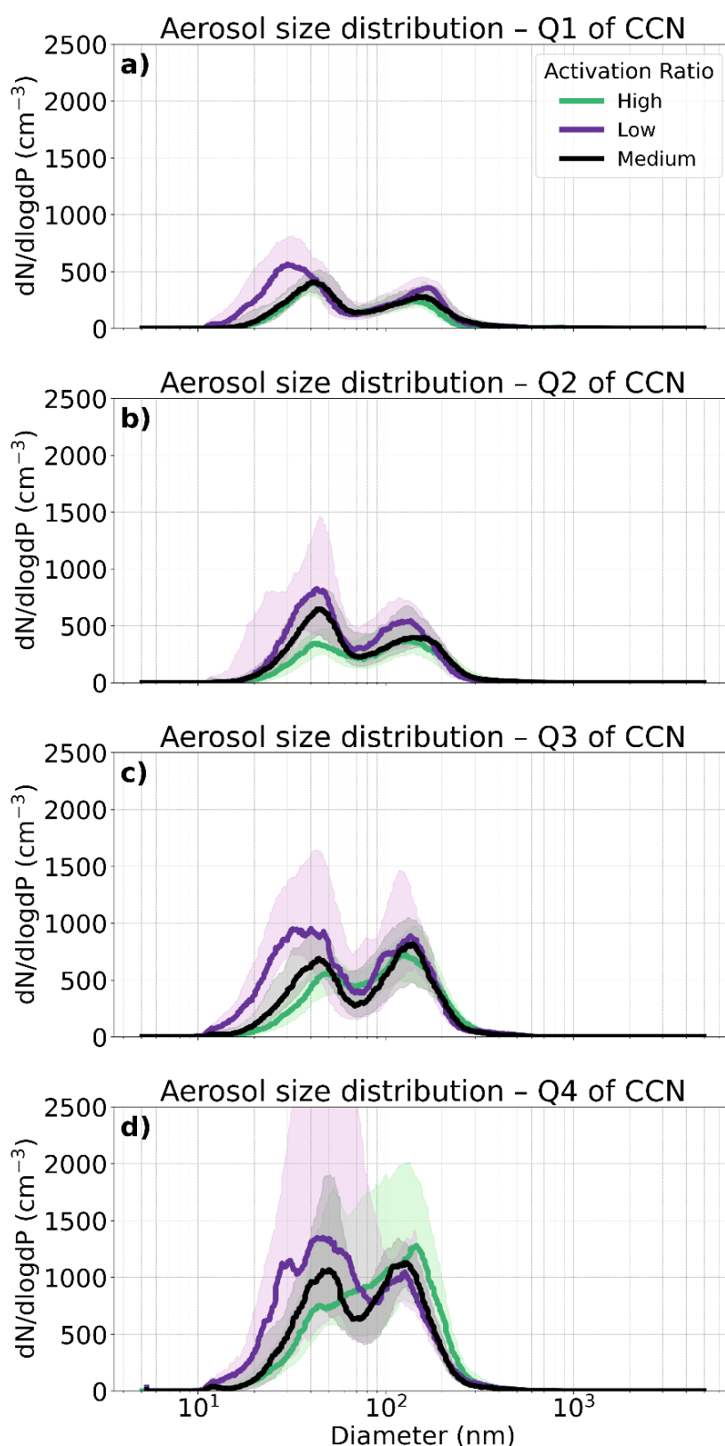
867 Figure 3: Aerosol size distributions for the four quartiles of CCN concentrations (a, b, c, d). Aerosol size 868 distributions are coloured by the relative values of activation ratio (Low – purple, Medium – black, 869 High– green). Shaded areas present the interquartile ranges. Values of activation ratio ranges for each 870 CCN concentration quartile as well as values of CCN concentration quartile are listed in Table S2.
