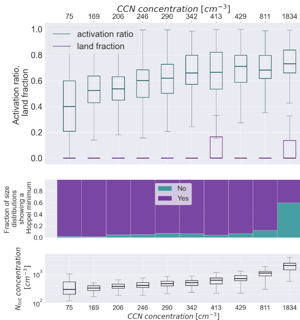
Figure 2: Activation ratio, land fraction, and fraction of data with no Hopple minimum present as well as total number concentration of particles for different CCN concentration bins. CCN concentration bins were created based on CCN concentration quantiles, ensuring equal distribution of data points between analysed bins. Values of activation ratio, land fraction, and total number concentration of particles are visualized by boxplots in which the middle line represents the median value, the upper and lower edges of a box show 75 % and 25% percentiles, and the whiskers show the entire range.
