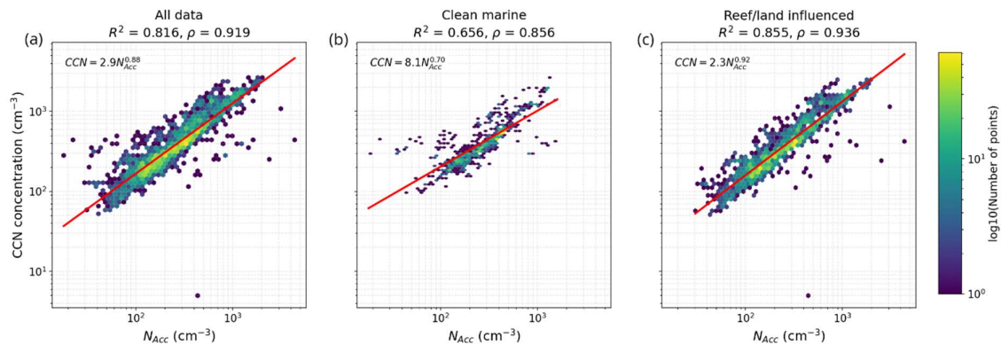
475 Figure 5: An ordinary least squares regression analysis fitted to log-log accumulation mode ( N_{Acc} ) and 476 CCN concentration data for all the data (a), clean marine data (b), and reef/land influenced data.
