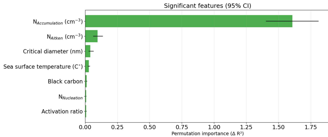
469 Figure 4: Permutation feature importance of climate variables in explaining CCN concentration. The 470 differences between original and permuted mean square errors on the x-axis indicate how important 471 each feature is in predicting the CCN concentration, with larger difference between original and 472 permuted values indicating a more important feature. The black whiskers indicate 95% confidence 473 intervals. The number of permutations used was 10000.
